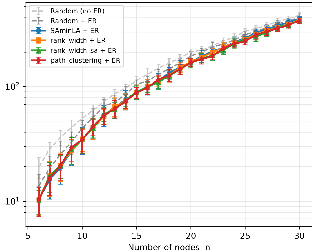
Total gates
