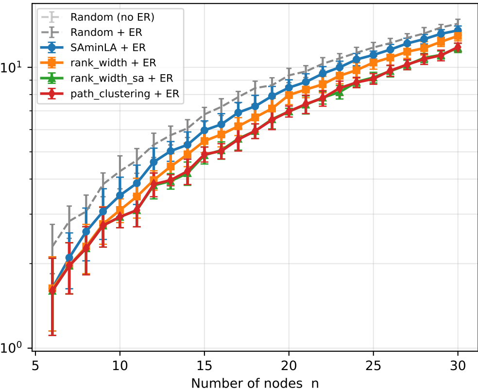
Emitters
