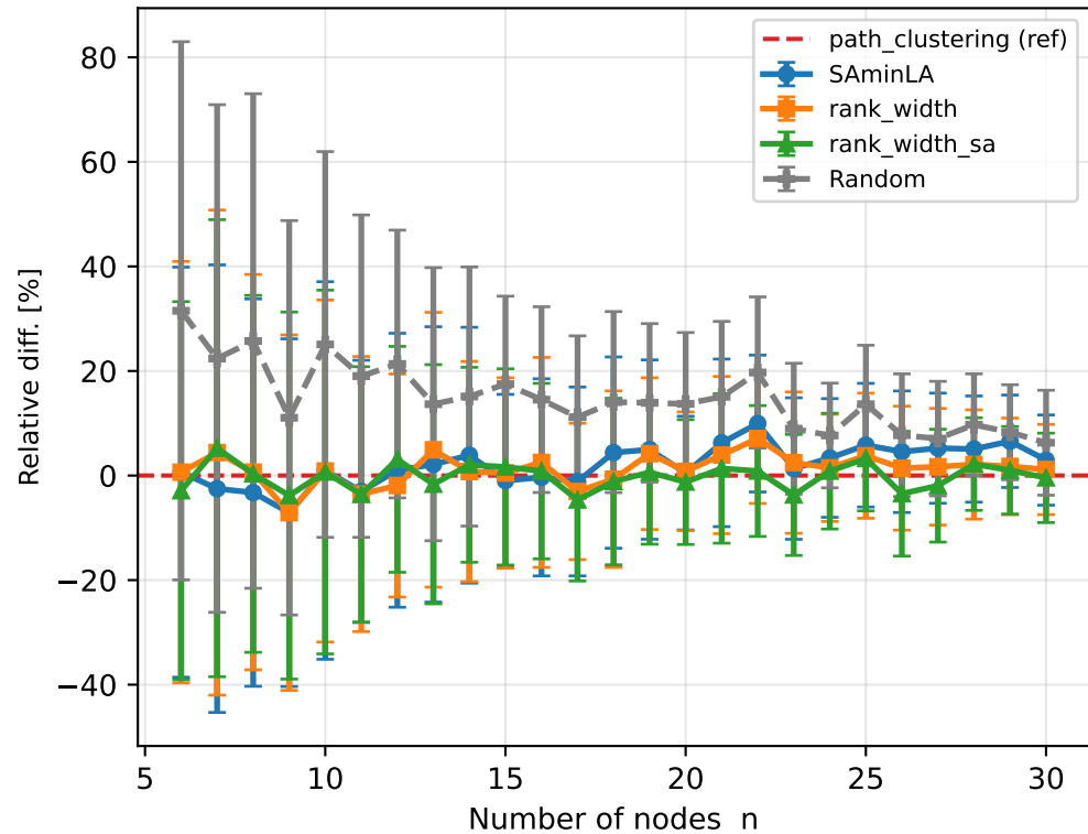
Total gates
