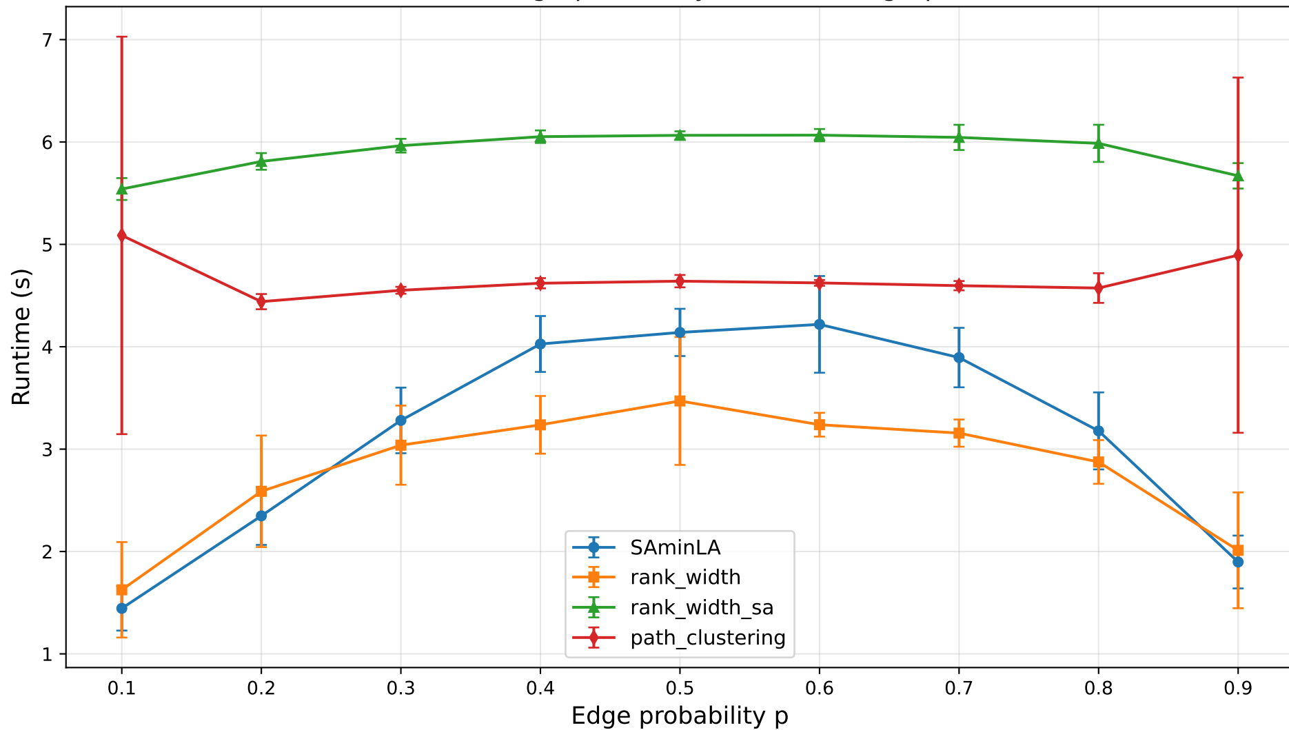
Runtime vs graph density (n = 20, ER graphs)
