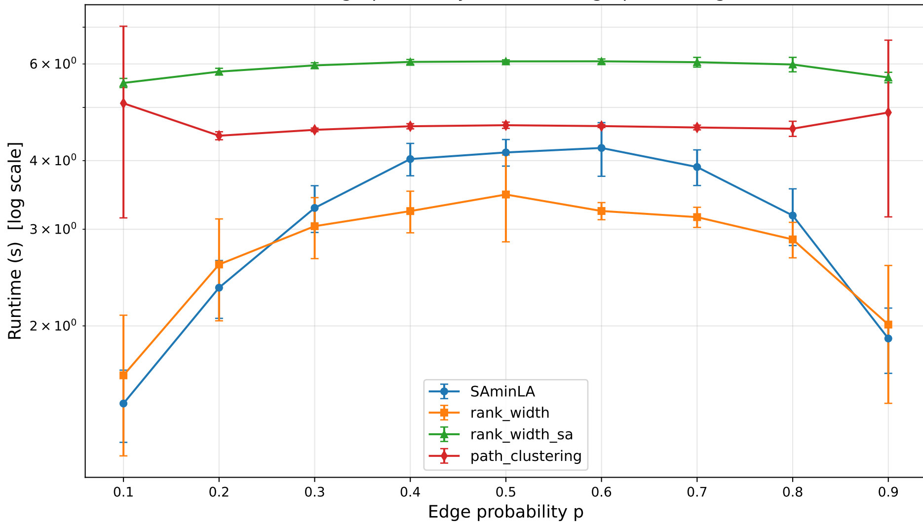
Runtime vs graph density (n = 20, ER graphs) — log scale
