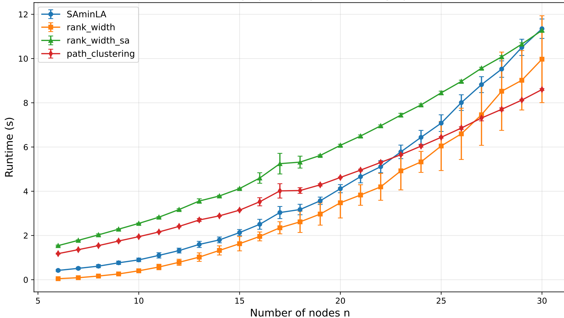
Runtime vs graph size (p = 0.65, ER graphs)
