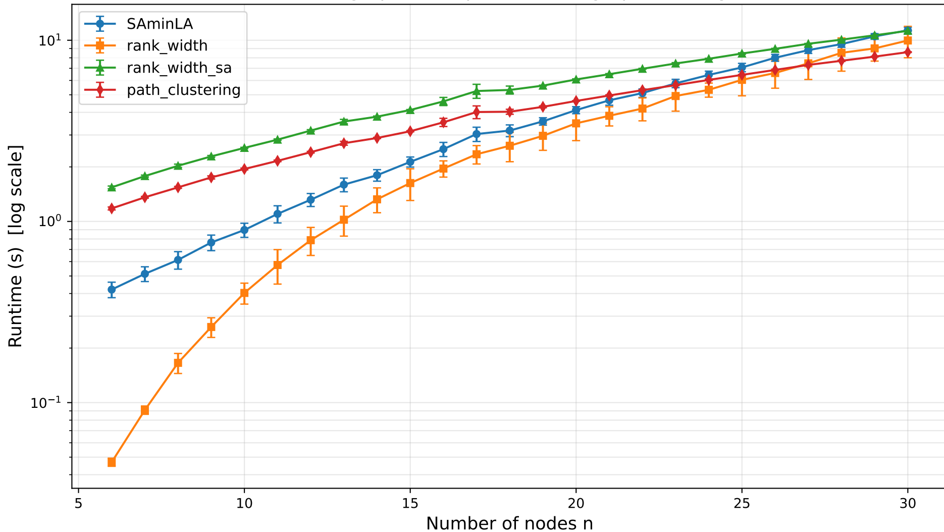
Runtime vs graph size ( p = 0.65 , ER graphs) — log scale
