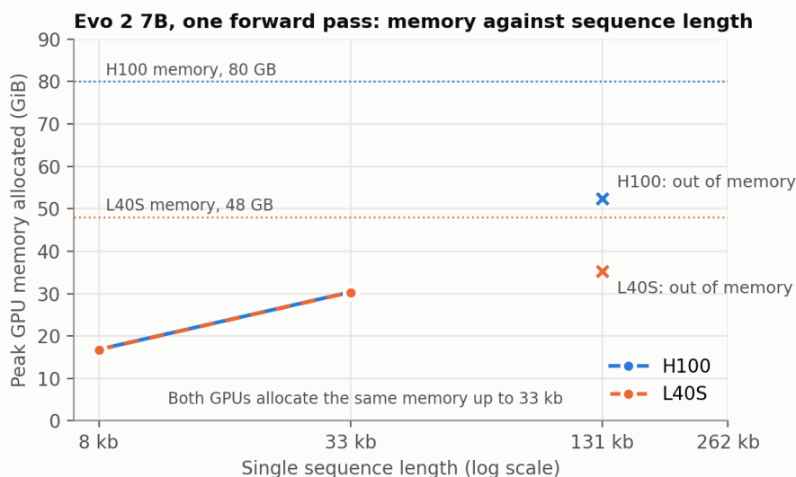
Figure 3: Peak GPU memory for one forward pass against sequence length. Crosses mark the memory in use when the next allocation failed. Dotted lines show nominal capacity (80 and 48 GB); PyTorch reported 79.2 and 44.4 GiB usable.
