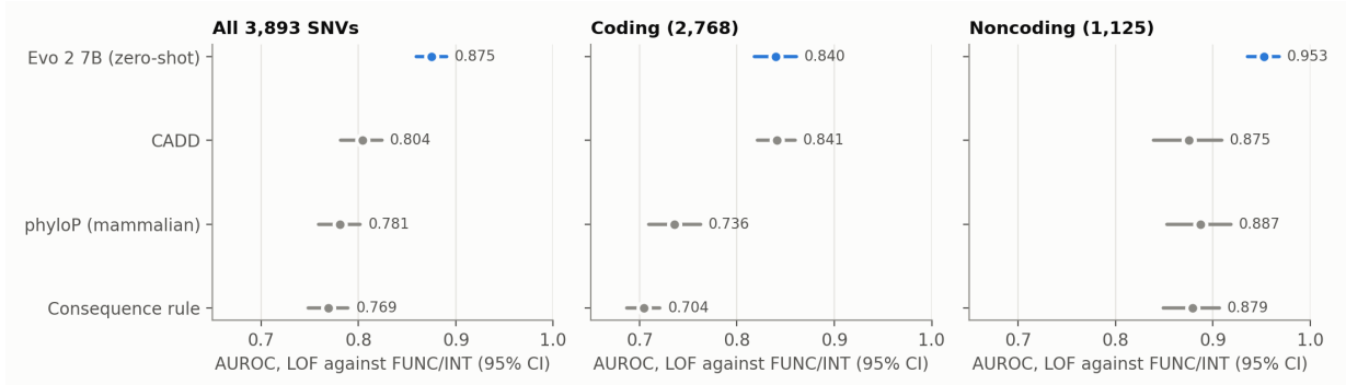
Figure 2: AUROC for BRCA1 loss-of-function variants with 95% grouped bootstrap intervals, reference platform. Baseline scores (CADD v1.3, mammalian phyloP) come from the Findlay et al. table.
