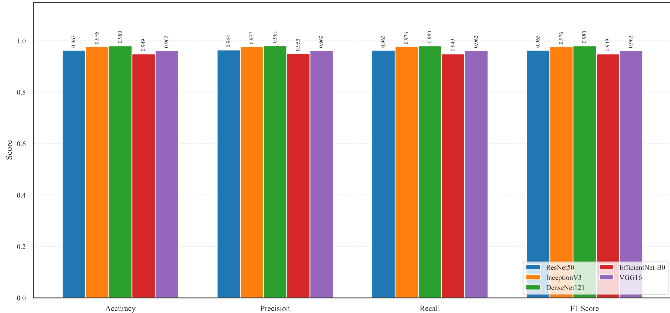
Model Performance Comparison (Test Set)
