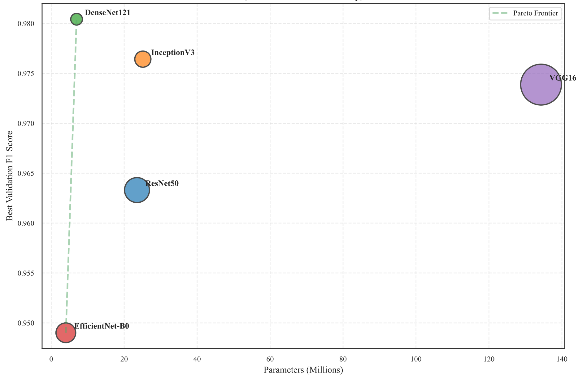
Model Efficiency: F1 Score vs Model Size (Marker size \propto 1/\text{Latency} )
