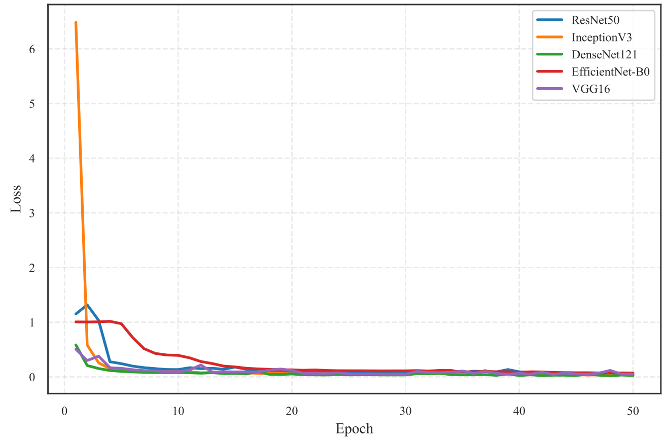
Validation Loss
