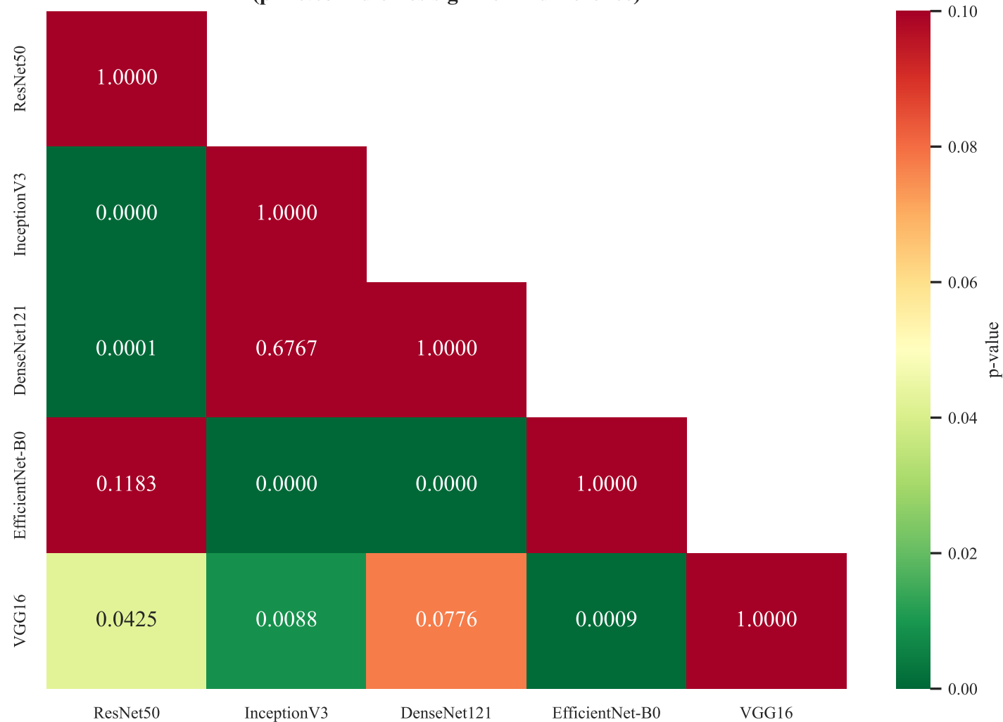
McNemar's Test p-values ( p < 0.05 indicates significant difference)
