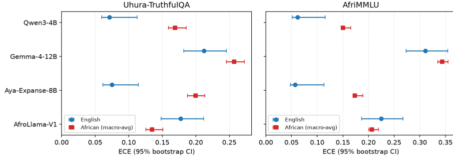
Figure 8: Bootstrap 95% confidence intervals for ECE by model, English versus African languages (markers are point estimates, bars are 95% intervals). For most general-purpose model and dataset pairs the African interval lies above the English interval and the two are disjoint; the exception is Gemma-4-12B on AfriMMLU, whose intervals overlap because it is already poorly calibrated in English.
