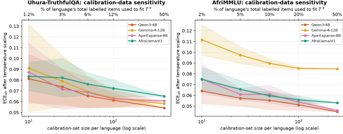
Figure 7: Macro-averaged African-language ECE after per-language temperature scaling versus calibration-set size per language (bottom axis, log scale; top axis, percentage of the language’s labelled items). Bands are \pm 1 standard deviation over 30 random subsamples at each size (zero width at “full,” the fixed 50% calibration split used throughout). Most of the achievable ECE reduction is already present by n_{\text{cal}} = 25 to 50.
