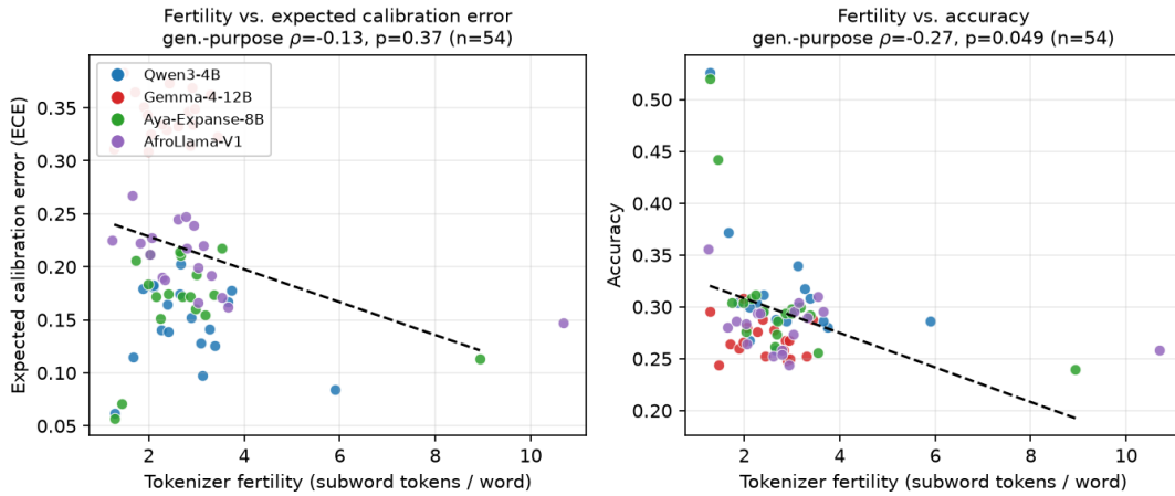
Figure 9: Tokenizer fertility versus ECE (left) and accuracy (right) on AfriMMLU, one point per model and language (each model uses its own tokenizer). Fertility is unrelated to ECE for the general-purpose models; the weak negative accuracy trend (right) is not robust to removing Amharic (see text). Dashed line: least-squares fit over the general-purpose models.
