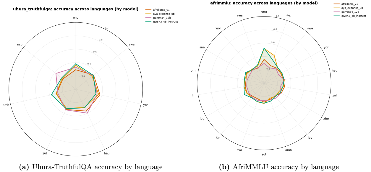
Figure 4: Accuracy across languages by model. Long English and French spokes collapse toward chance across African languages.
