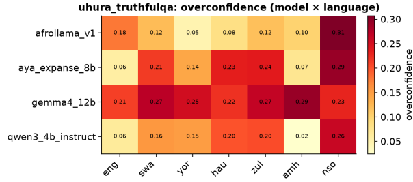
(a) Uhura-TruthfulQA overconfidence by language
