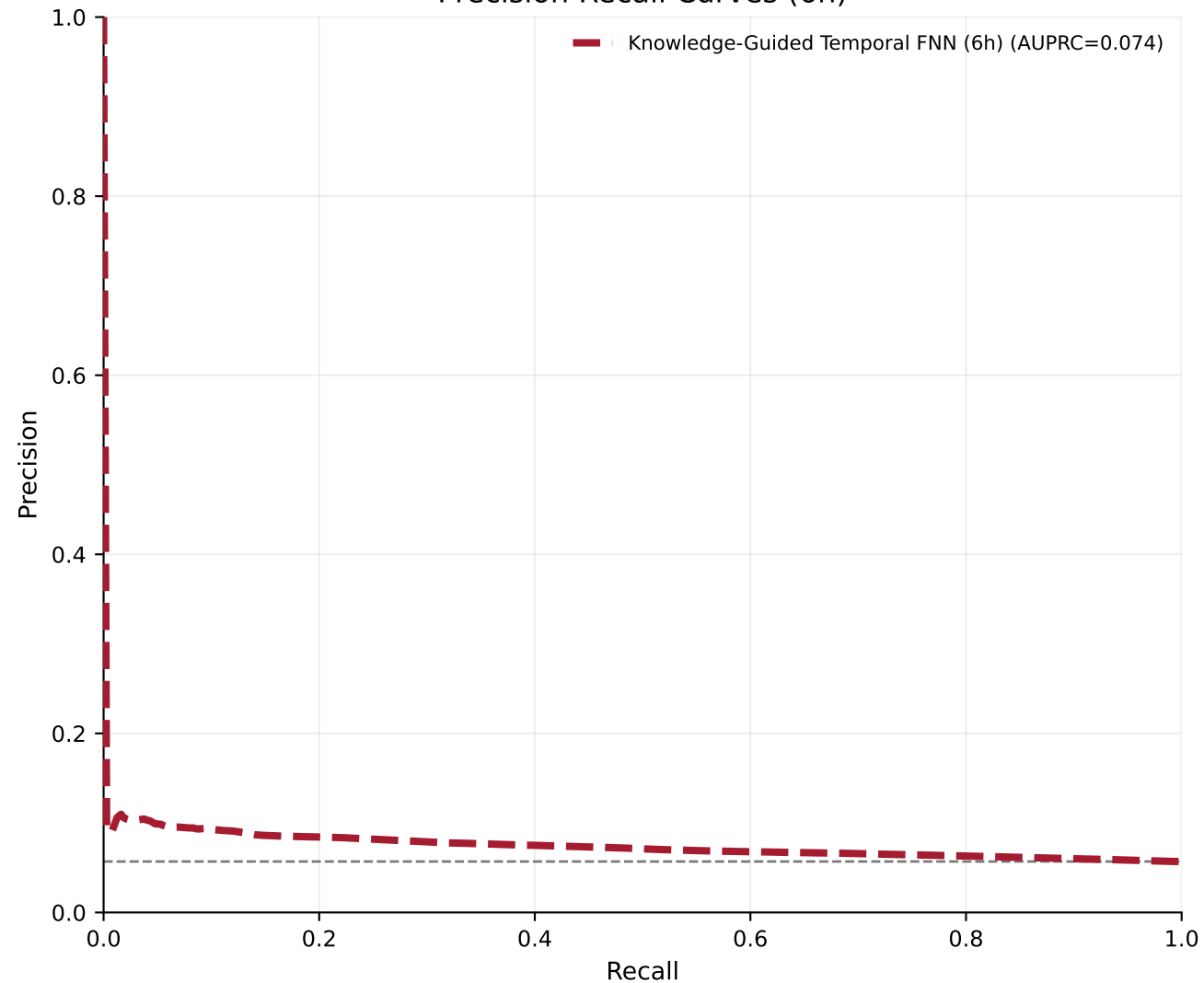
Precision Recall Curves (6h)
