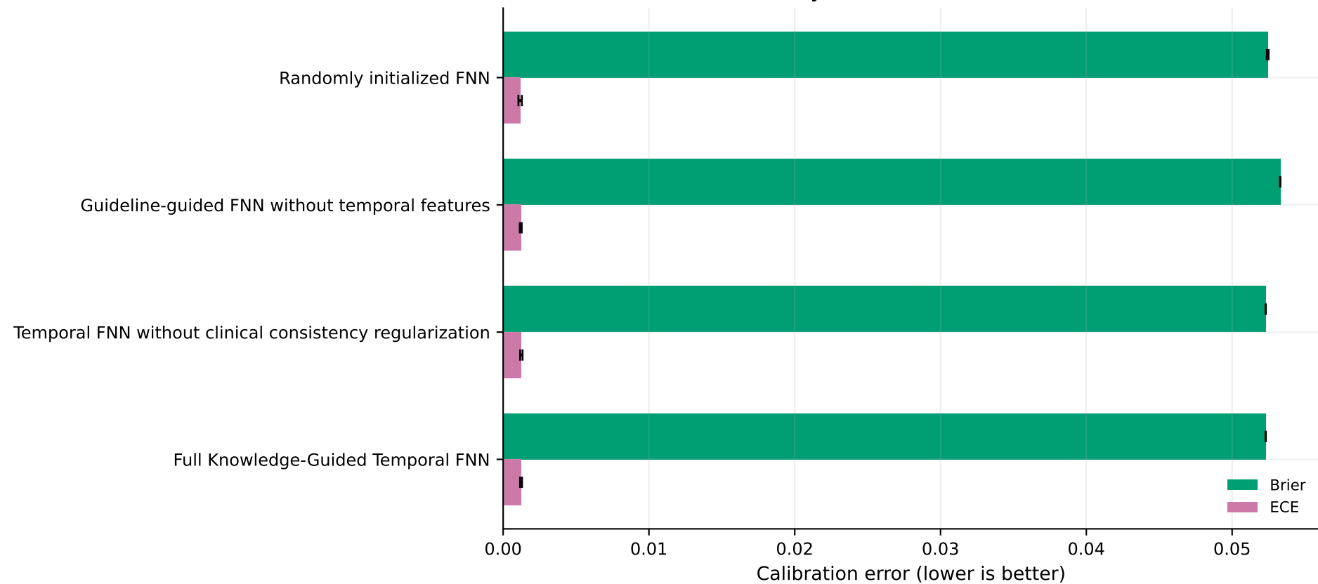
Ablation Study: Calibration (6-hour outcome)
