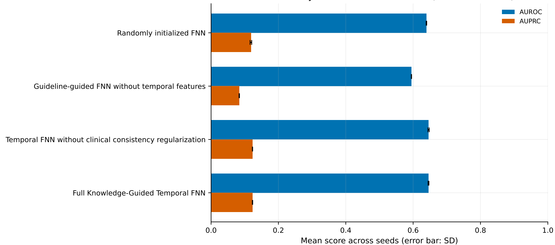
Ablation Study: Predictive Performance (6-hour outcome)
