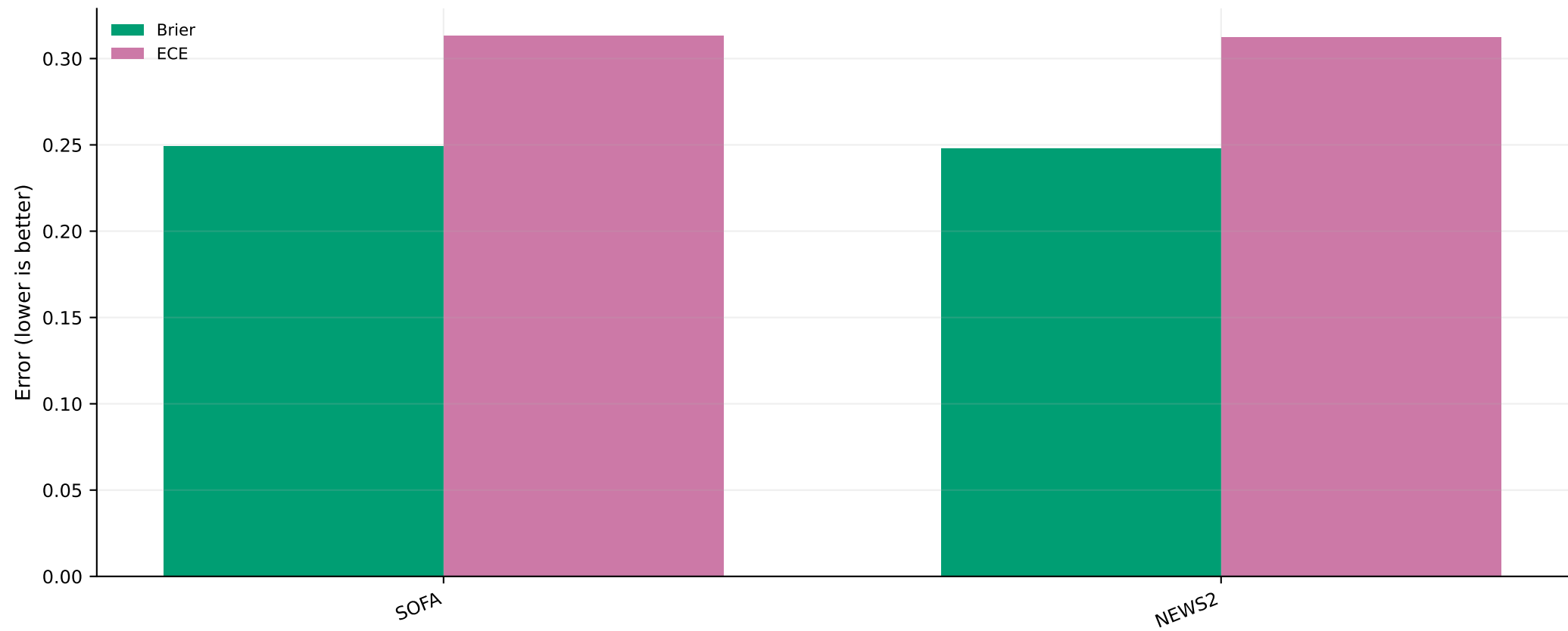
Calibration Error for 24-hour Prediction
