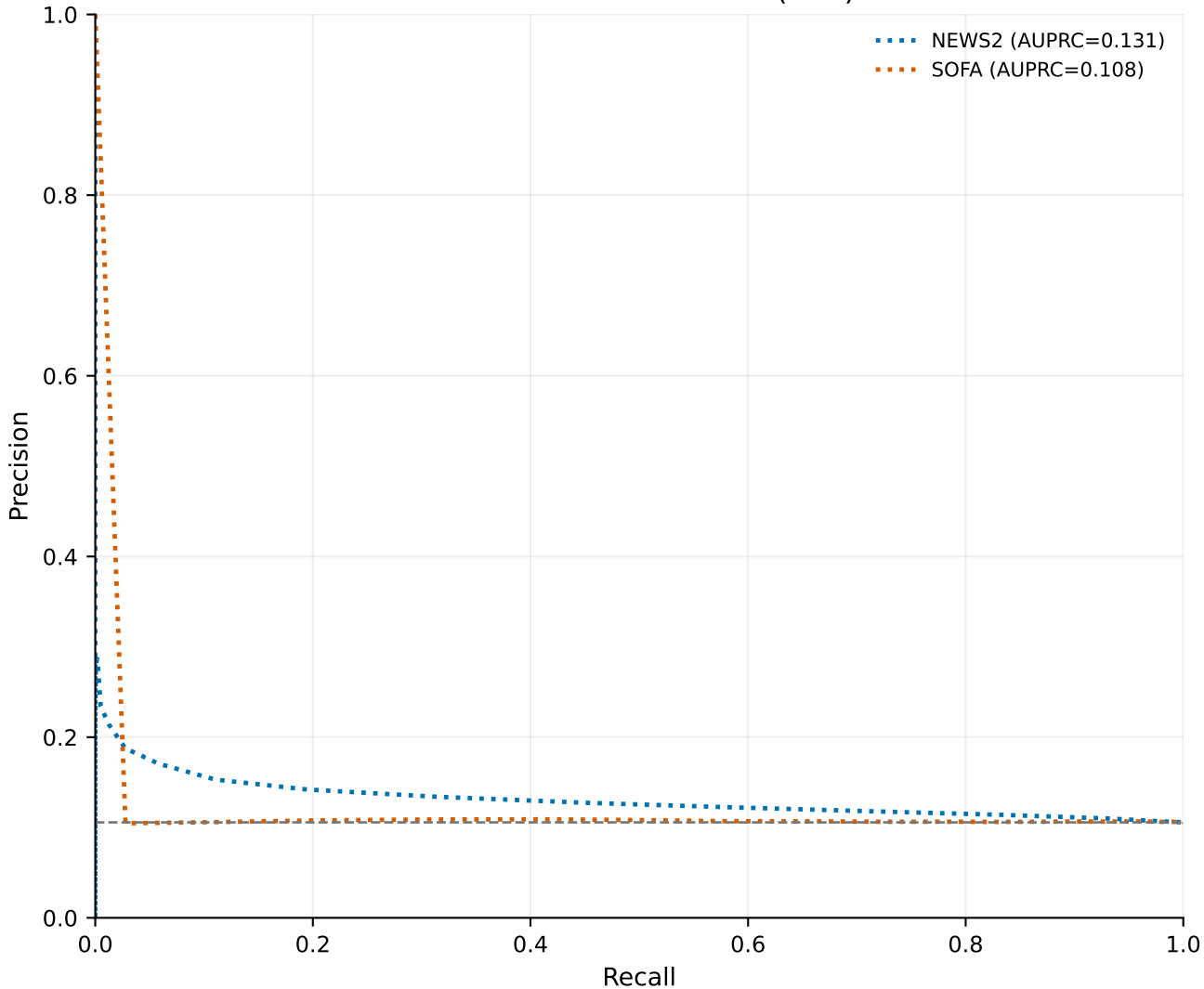
Precision Recall Curves (12h)
