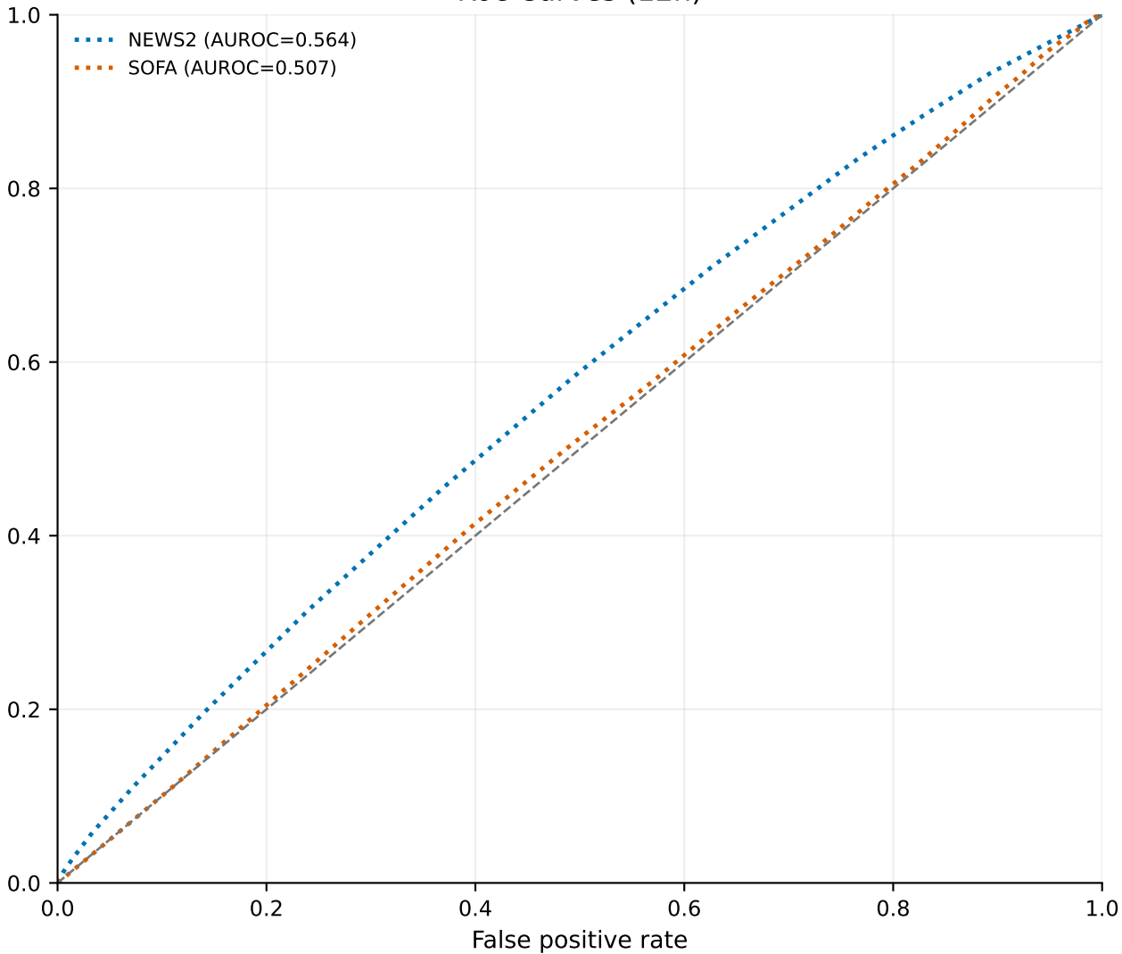
Roc Curves (12h)
