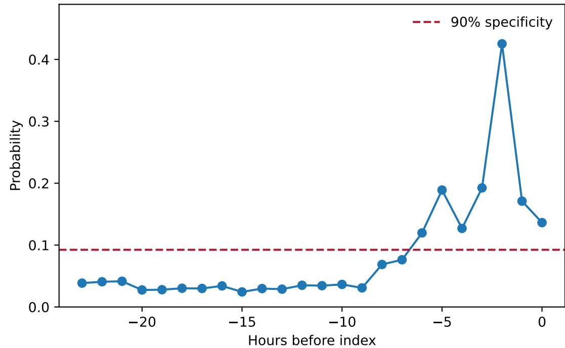
TP: largest physiologic changes
