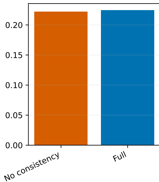
Normalized drift
