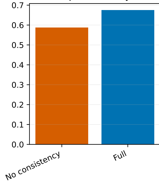
Top-10 stability
