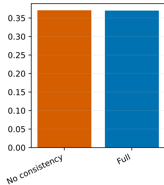
Violation rate
