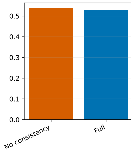
Guideline-risk rho
