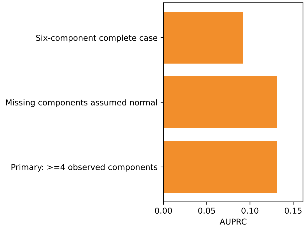
SOFA Outcome-Definition Sensitivity
