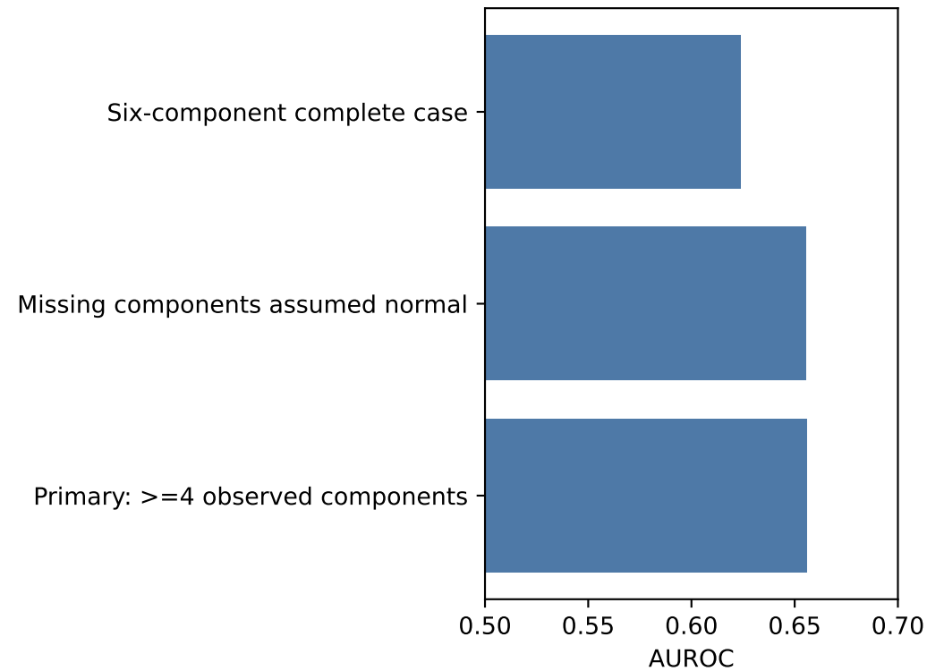
SOFA Outcome-Definition Sensitivity
