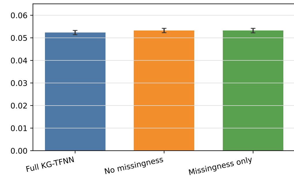
Brier score
