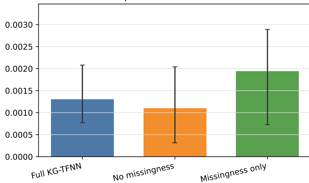
Expected calibration error
