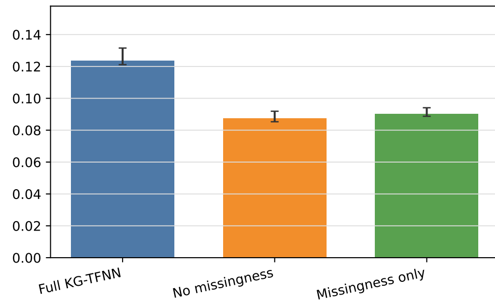
Expected calibration error
