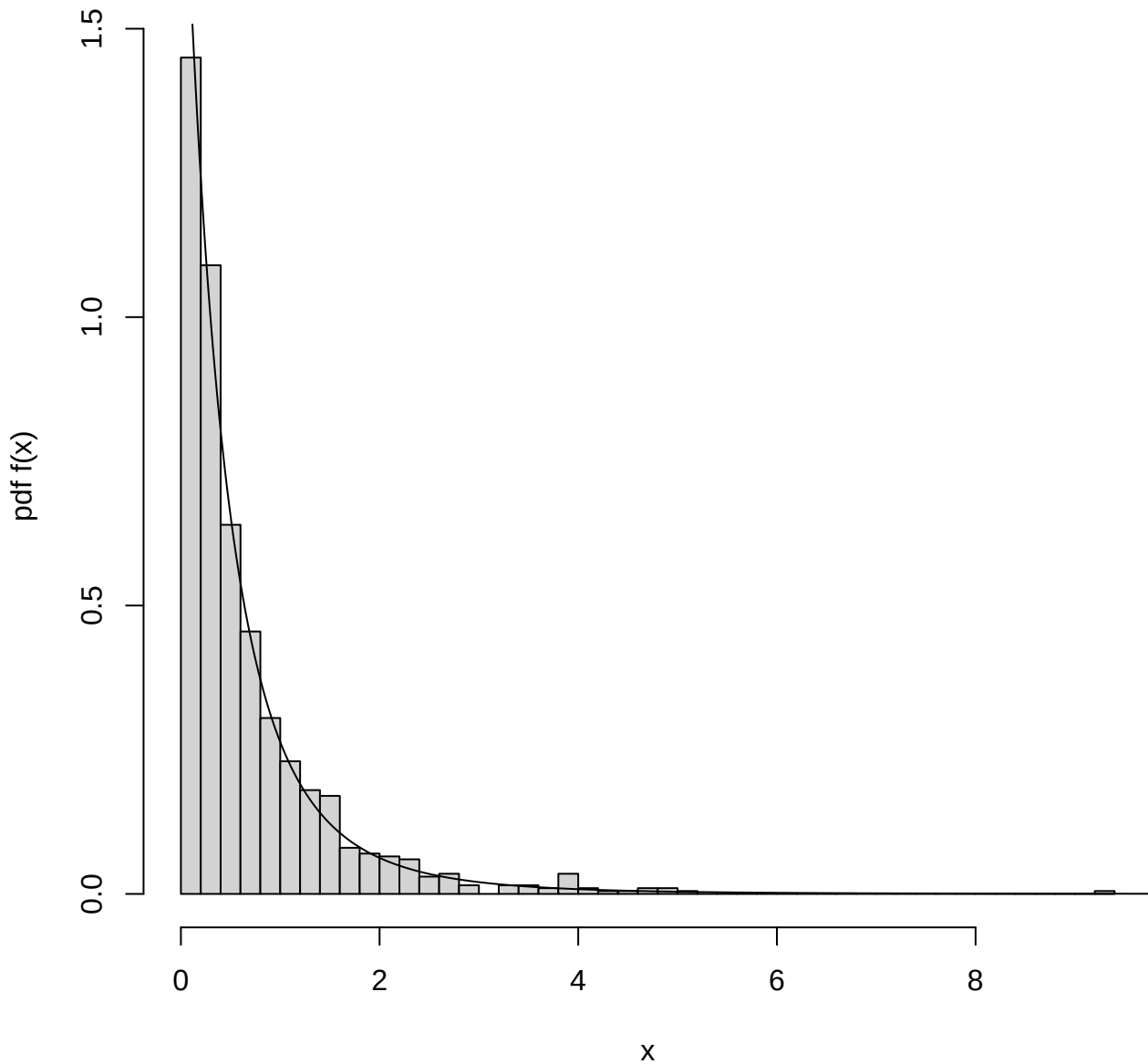
theoretical and simulated pareto(3, 2) density
