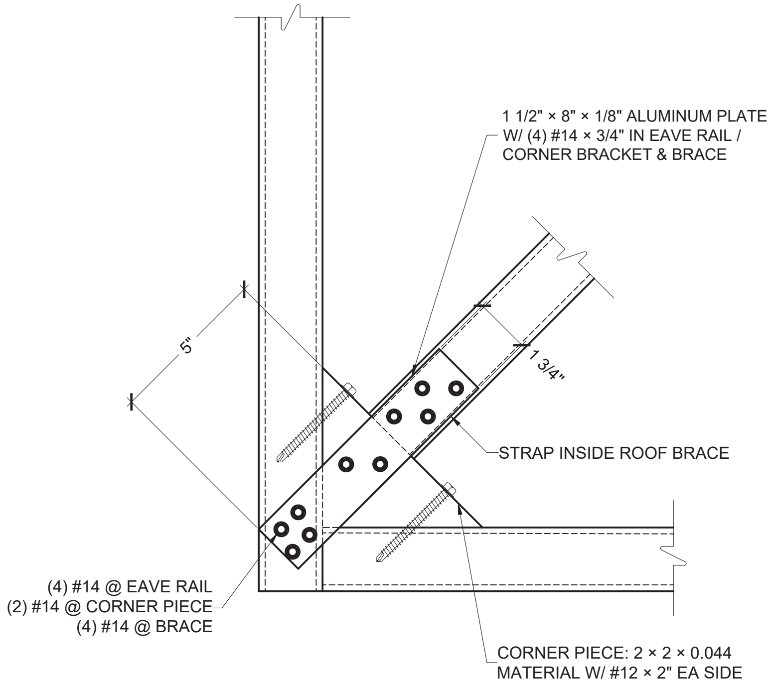
ROOF BRACING CONNECTION DETAIL SCALE: N.T.S.
