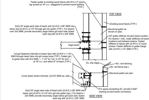
Beam to Gutter Connection SCALE: 3" = 1'-0"
