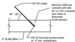
Cable to Foundation Connection SCALE: 3" = 1'-0"
