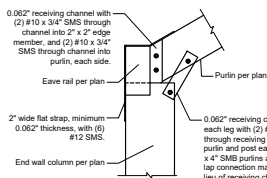
Roof Brace Connection SCALE: 3" = 1'-0"
