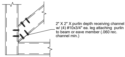
Roof Bracing Connection Detail
