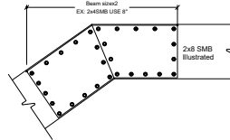
Gusset Connection SCALE: 2" = 1'-0"
