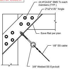
Cable to Frame Connection SCALE: 3" = 1'-0"
