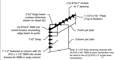
Sloped Purlin to Column Connection SCALE: 1 1/2" = 1'-0"
