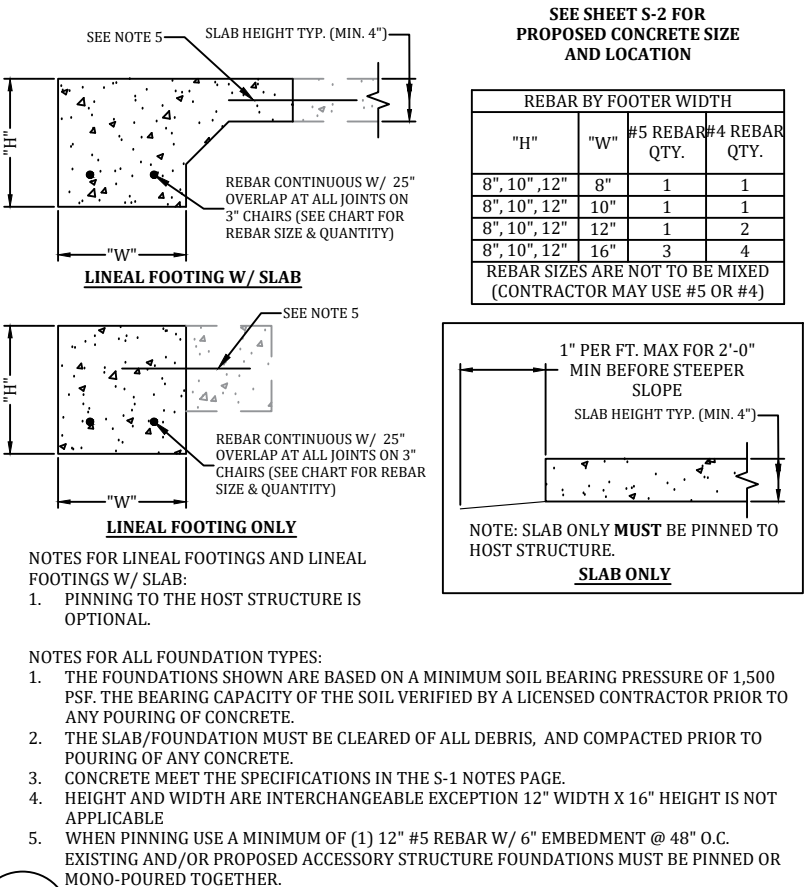
FOUNDATION DETAIL
