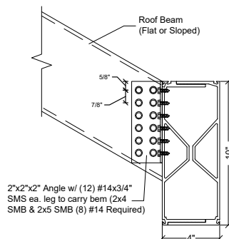
Roof Beam to Carrier Beam Connection Detail
