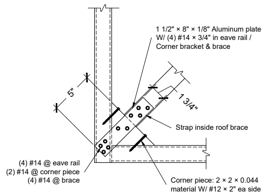
Roof Bracing Connection Detail
