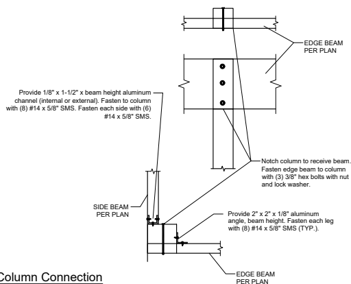
Beam to Column Connection
