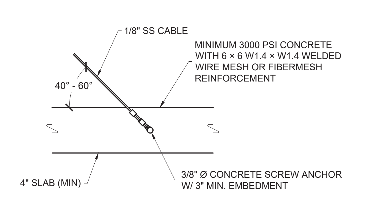
CABLE TO FOUNDATION CONNECTION SCALE: N.T.S.
