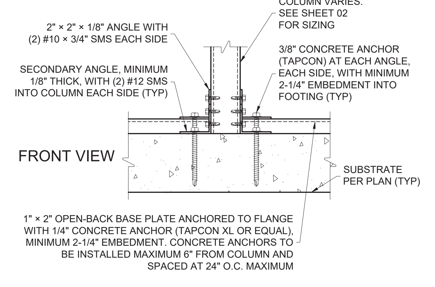
COLUMN TO FND CONNECTION FOR 2 × 4 OR LARGER SCALE: N.T.S.
