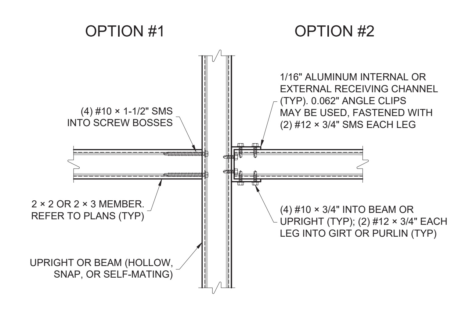
BEAM/POST TO GIRT/PURLIN CONNECTION SCALE: N.T.S.
