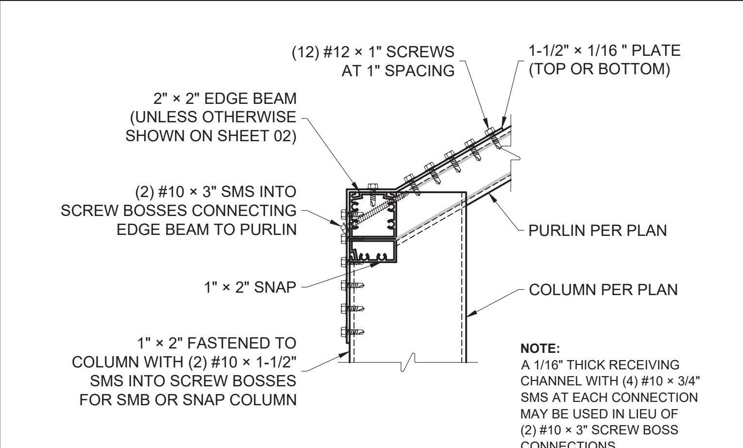
SLOPED PURLIN TO COLUMN CONNECTION SCALE: N.T.S.
