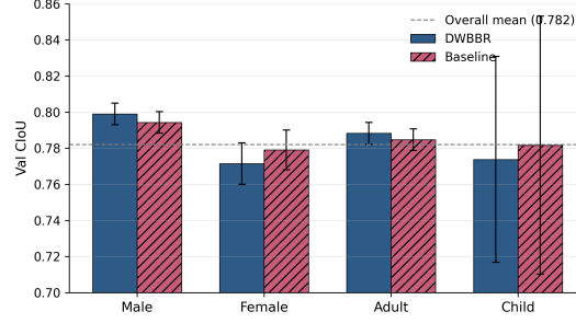
Fig. 4. Validation-set CIoU for DWBBR and the baseline, by demographic group.
