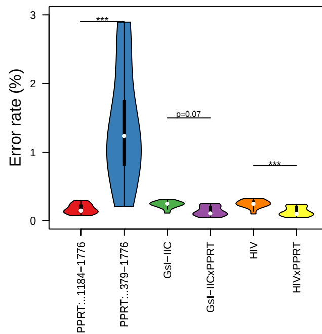
cDNA (middle)
