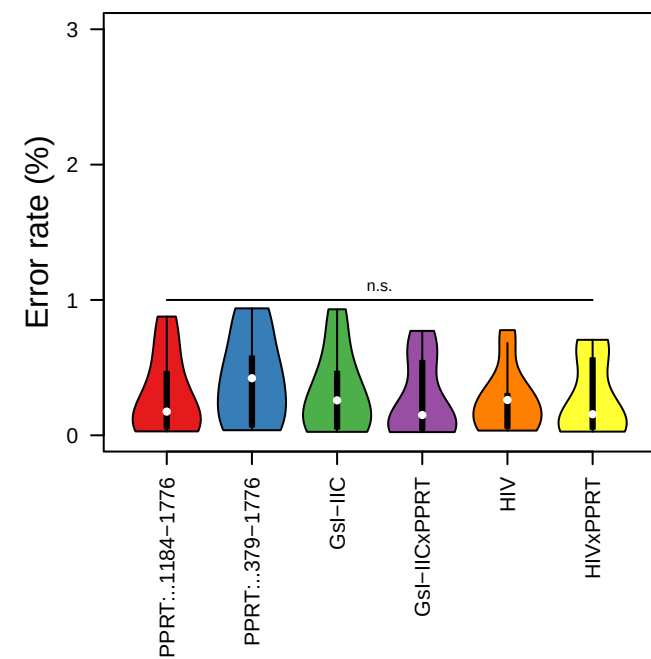
cDNA (5' end)
