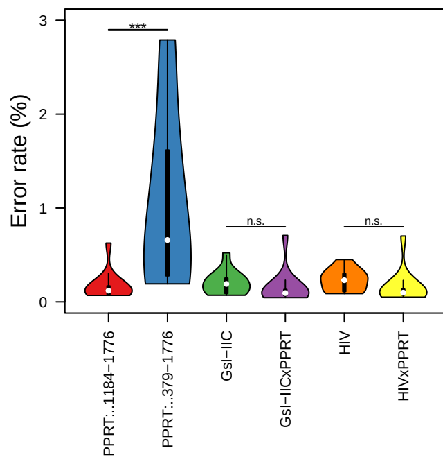
cDNA (3' end)
