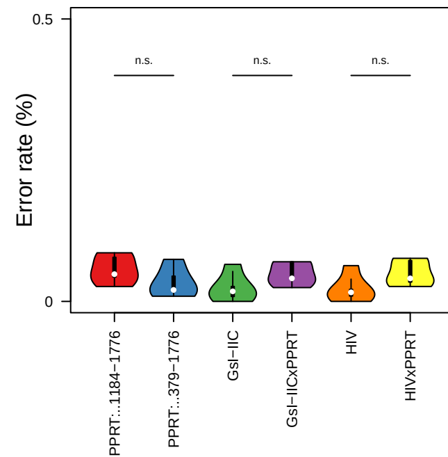
cDNA (5' end)
