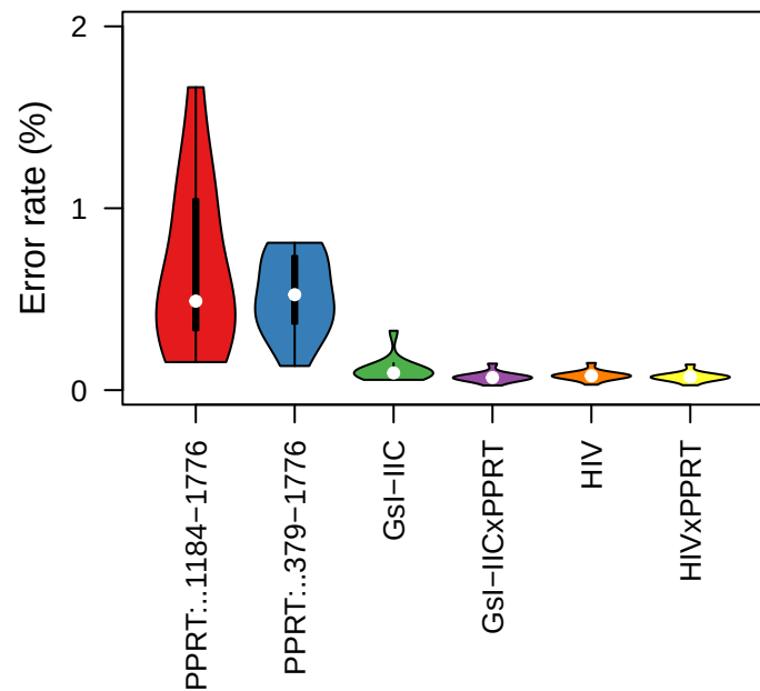
cDNA (middle)
