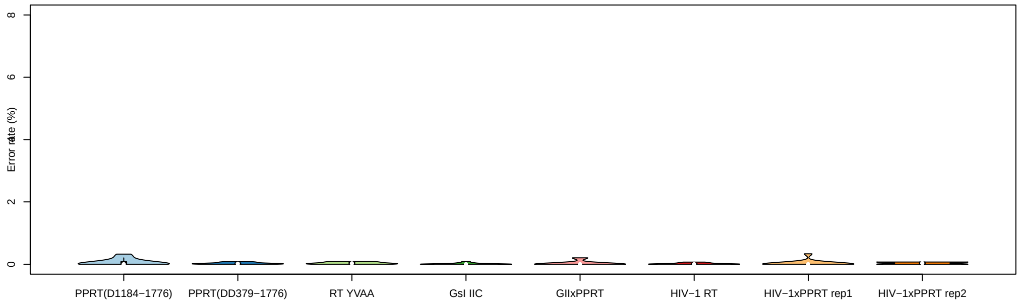
cDNA (5' end)
