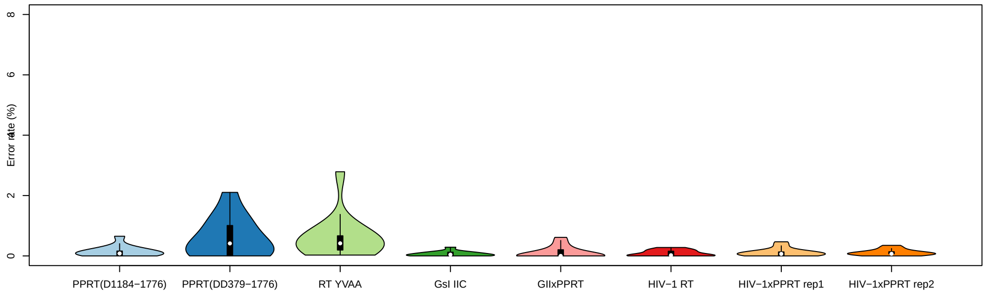
cDNA (middle)
