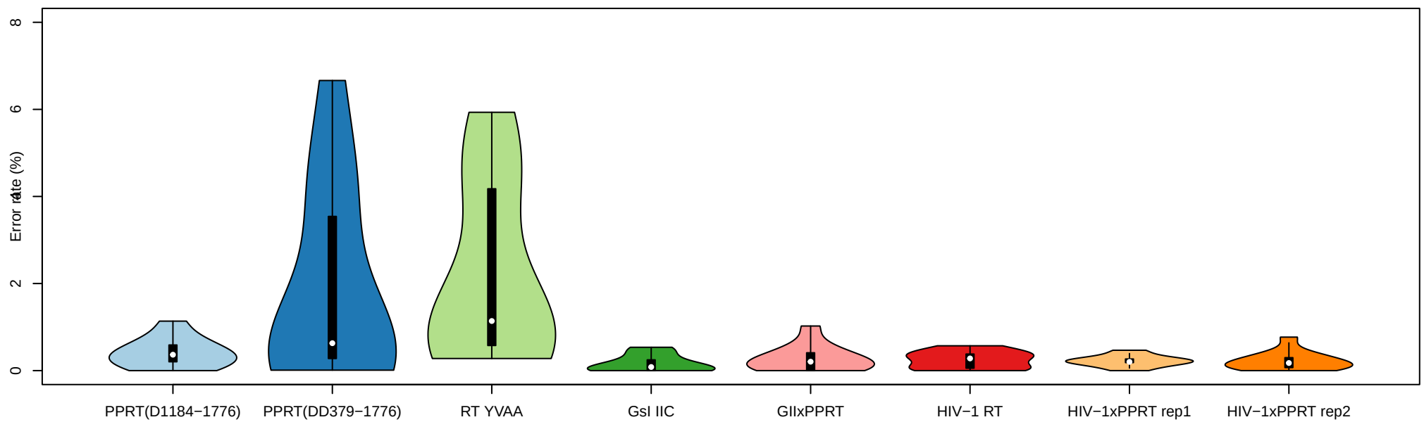
cDNA (3' end)
