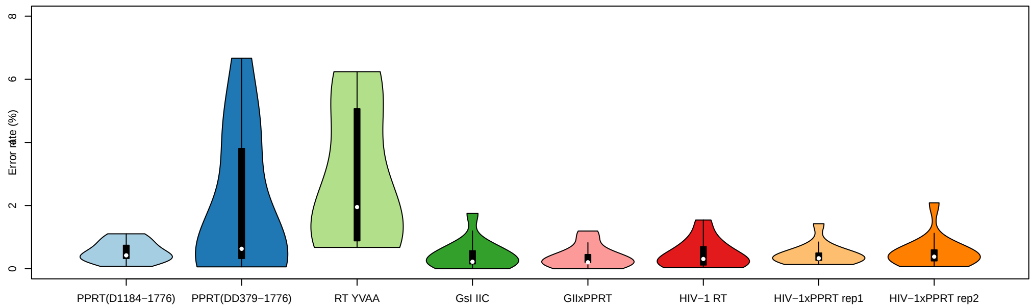
cDNA (3' end)
