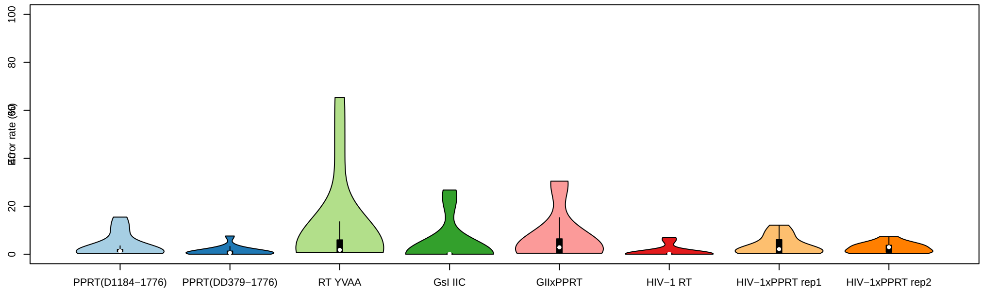
cDNA (middle)
