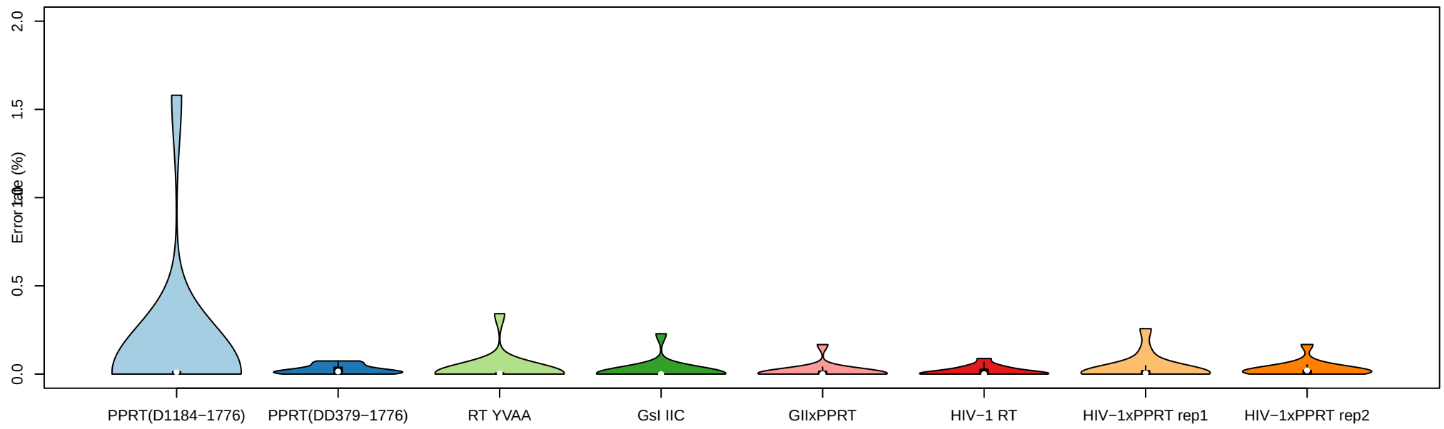
cDNA (5' end)
