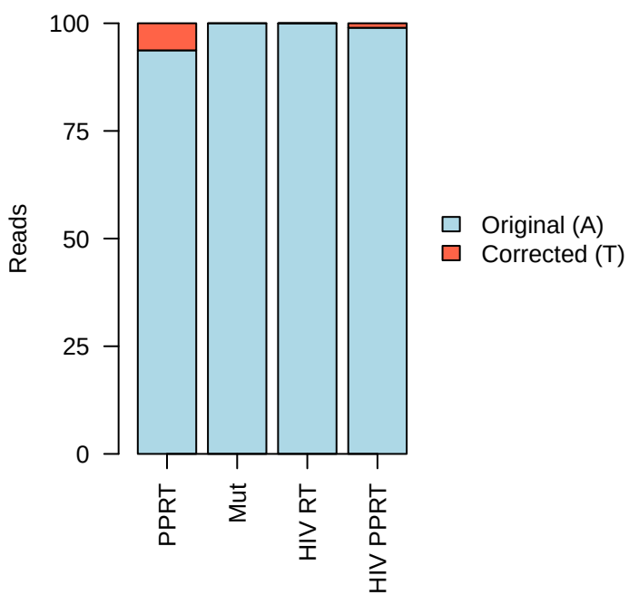
Mismatched nucleotide in unused primer
