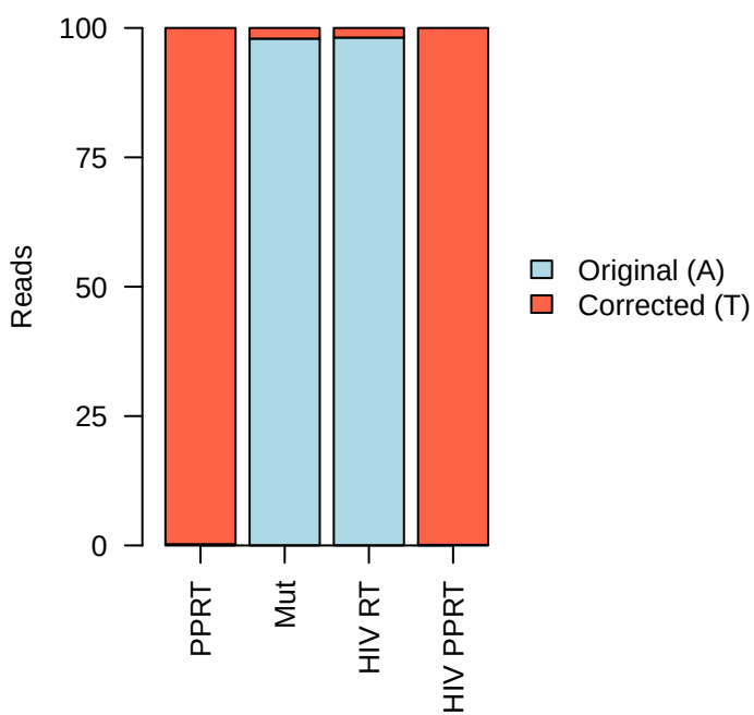
Mismatched nucleotide in extended primer
