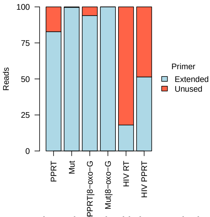
Mismatched nucleotide in unused primer
