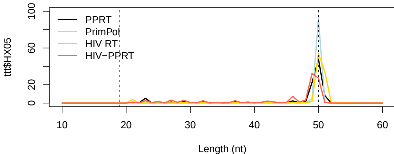
cDNA length distribution
