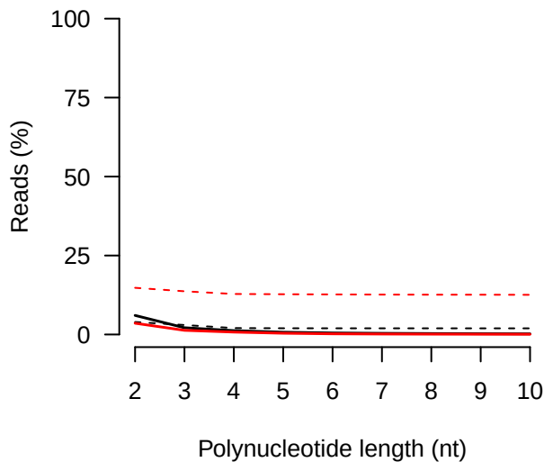
Reads end with polyT
