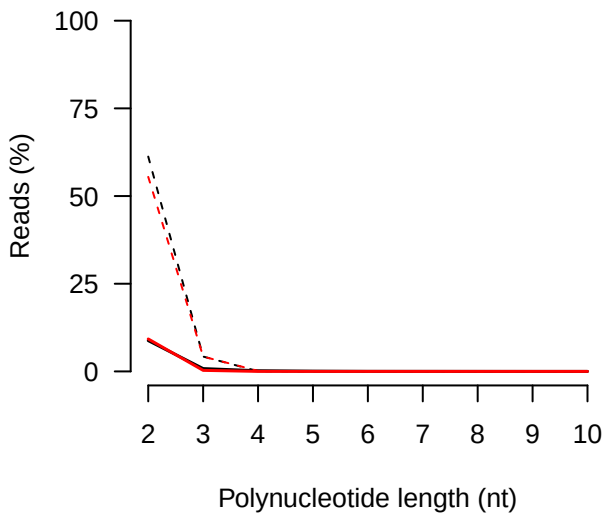
Reads end with polyG
