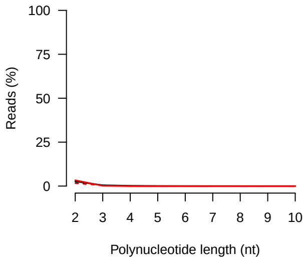
Reads end with polyC
