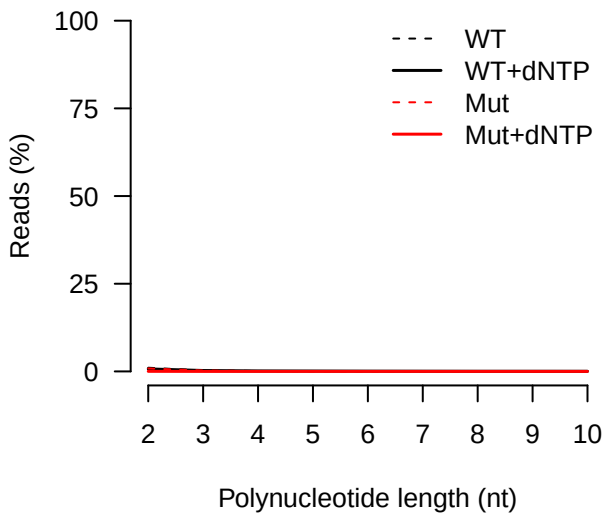
Reads end with polyA
