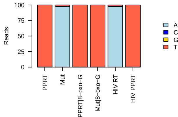
Nucleotide frequency at Pos31 (A)
