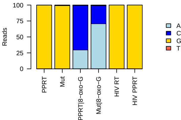
Nucleotide frequency at Pos28 (8-oxo-G)
