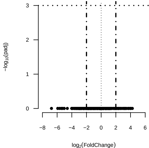
Mature miRNA
