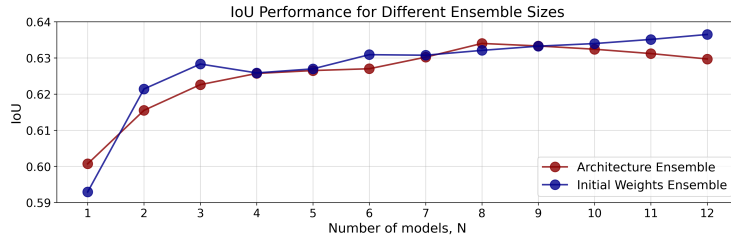
Figure 2: Ensemble IoU over all smoke densities as a function of ensemble size for two ensemble design schemes: random initial weights (blue) and archiecture-based (red).
