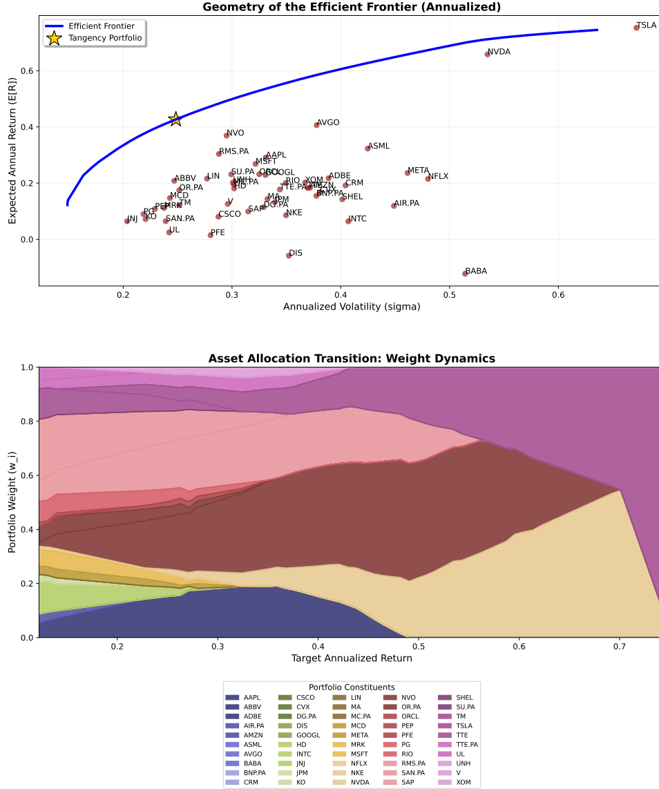
Figure 1: Efficient Frontier visualization.
