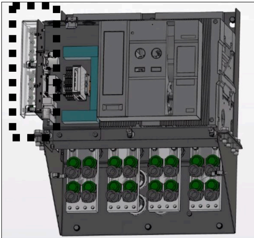
SWITCH DISCONNECTOR 2500A
