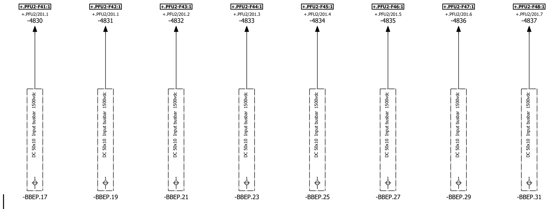
DC CONNECTION FROM PV SYSTEM TO DU INPUT BUSBARS 50x10 1500vdc
