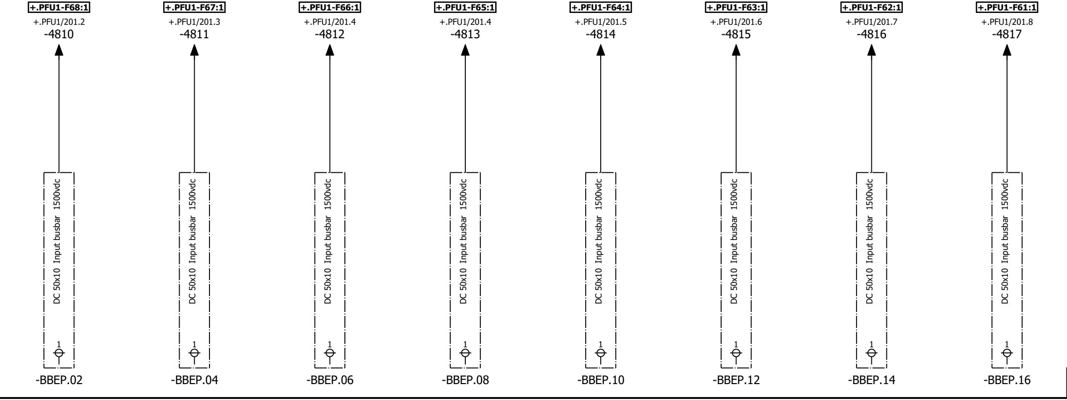
DC CONNECTION FROM PV SYSTEM TO DU INPUT BUSBARS 50x10 1500vdc
