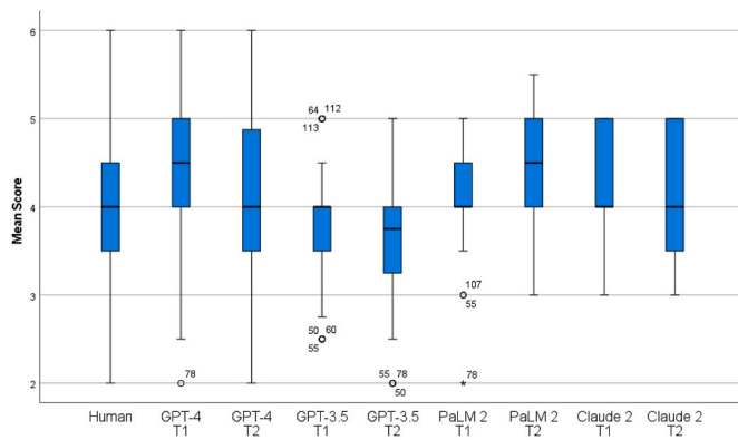
Fig. 2. Box plots for mean scores from humans and LLMs at T1 and T2.
