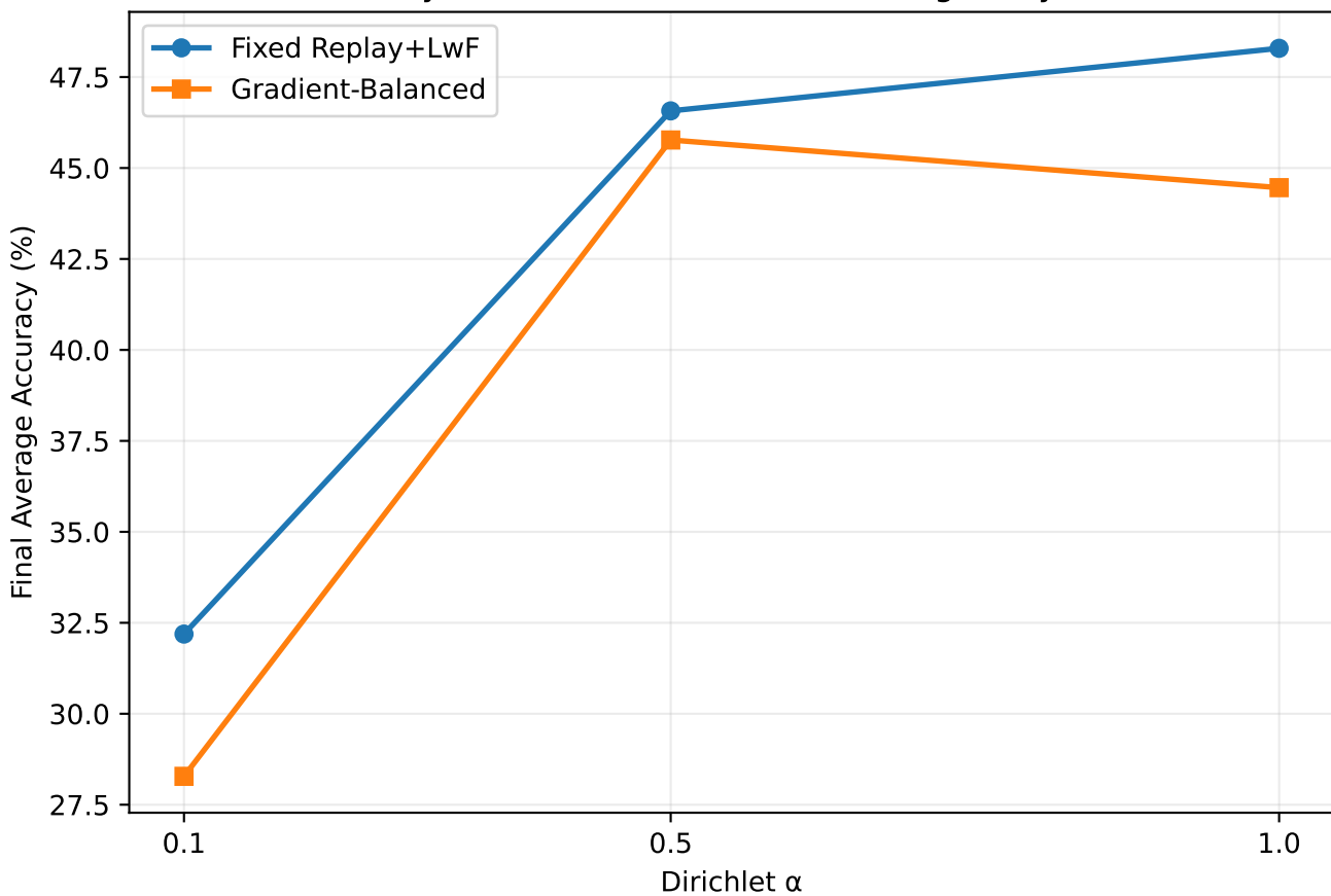
Accuracy Under Different Client Heterogeneity Levels
