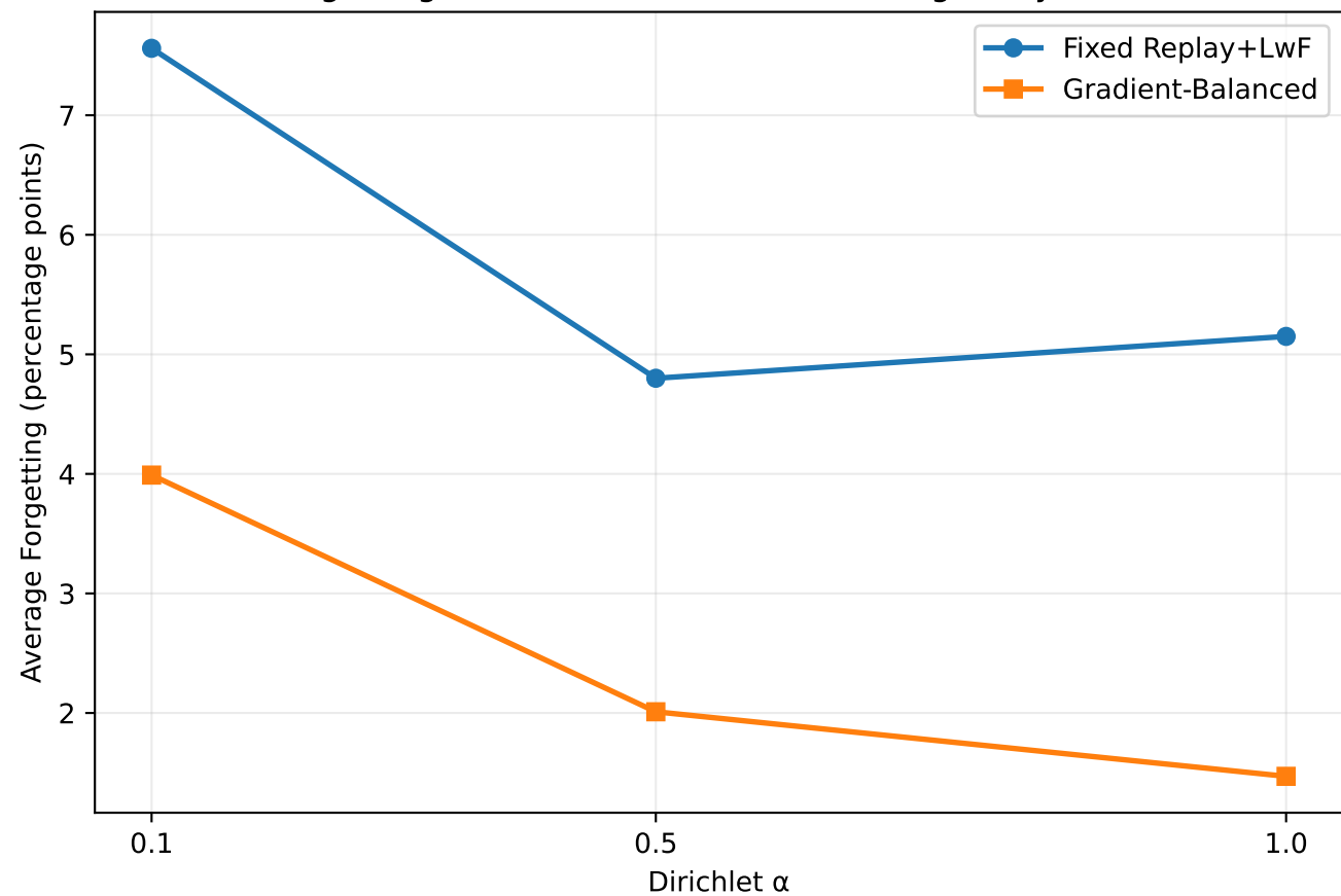
Forgetting Under Different Client Heterogeneity Levels
