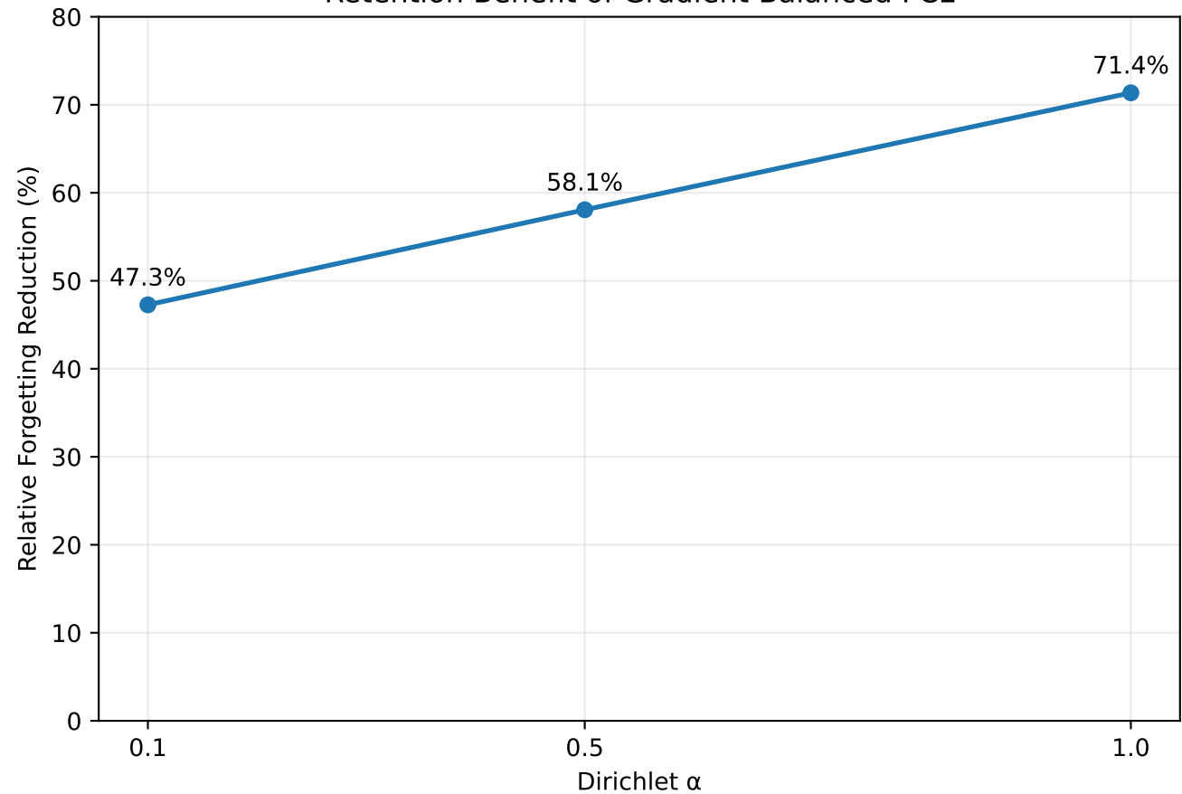
Retention Benefit of Gradient-Balanced FCL
