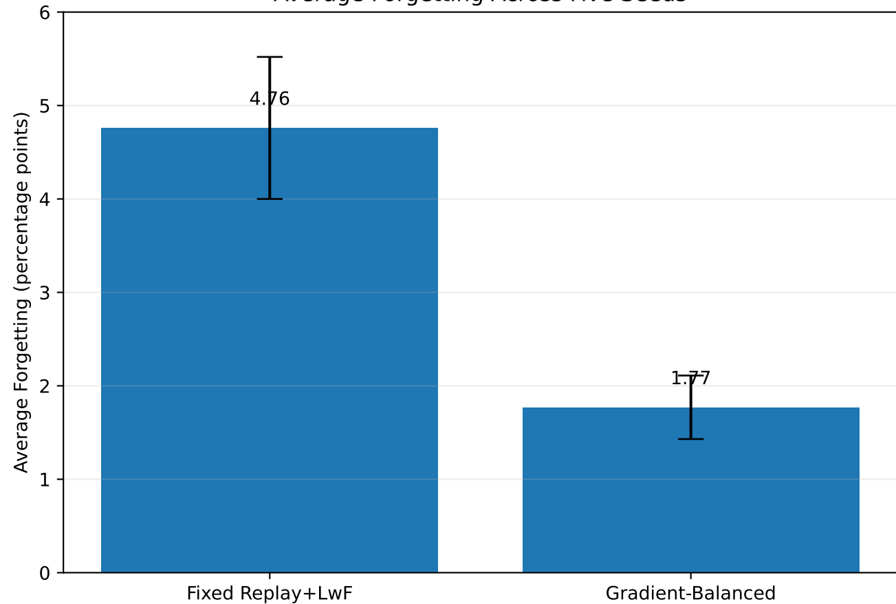
Average Forgetting Across Five Seeds
