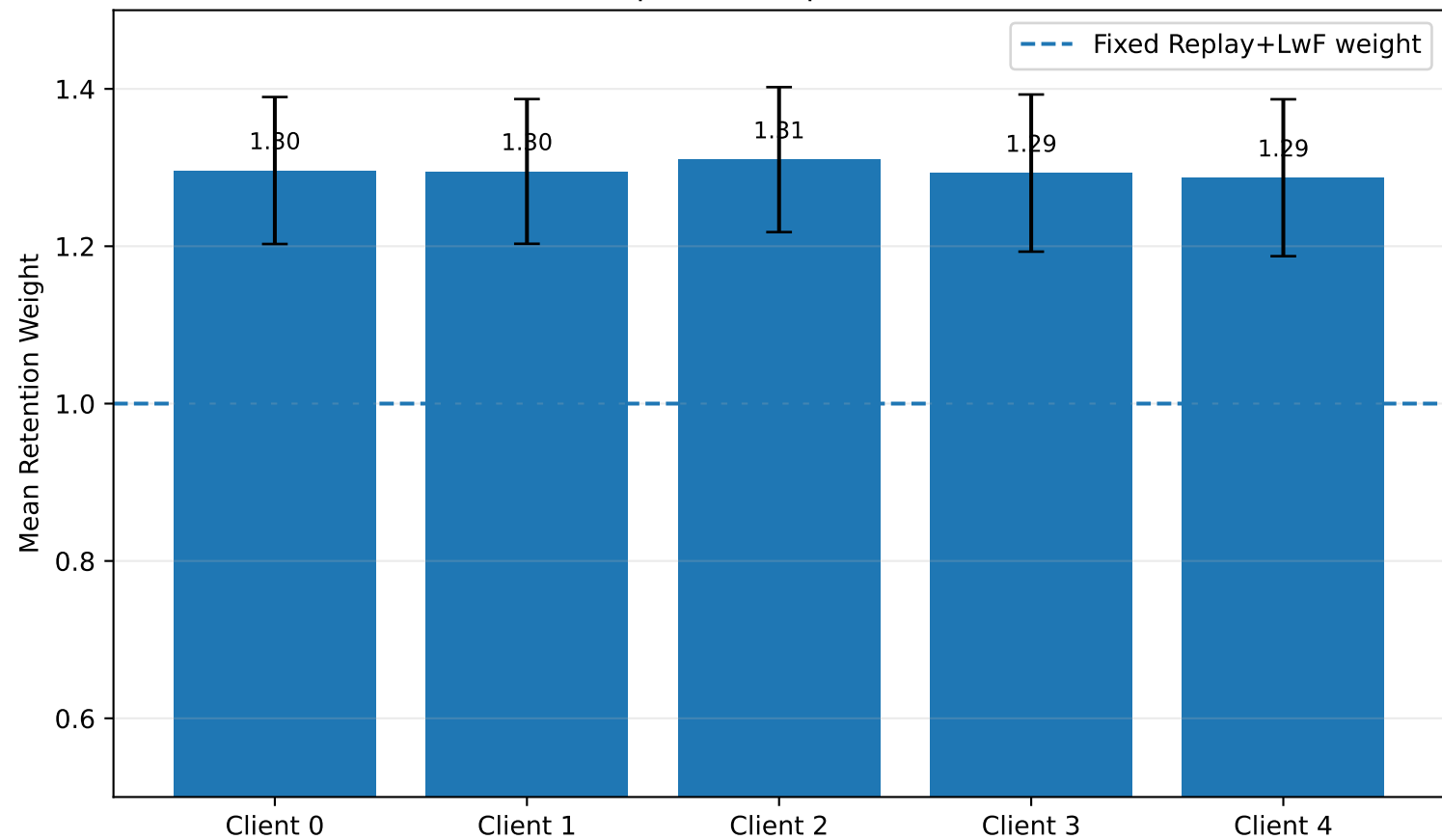
Client-Specific Adaptive Retention
