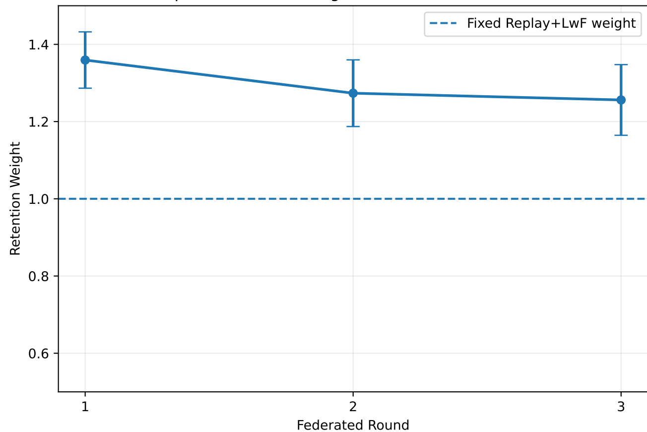
Adaptive Retention Weight Across Federated Rounds
