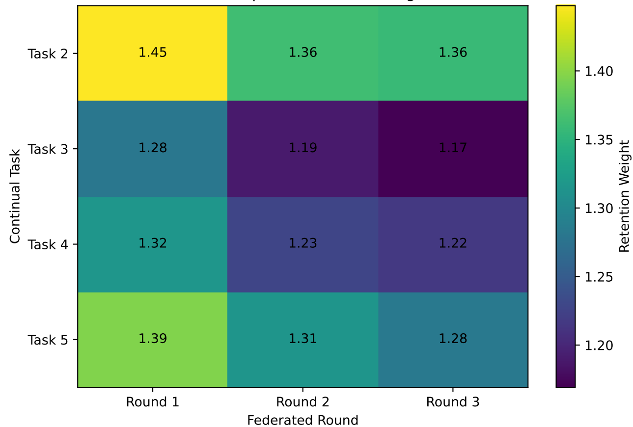
Mean Adaptive Retention Weight
