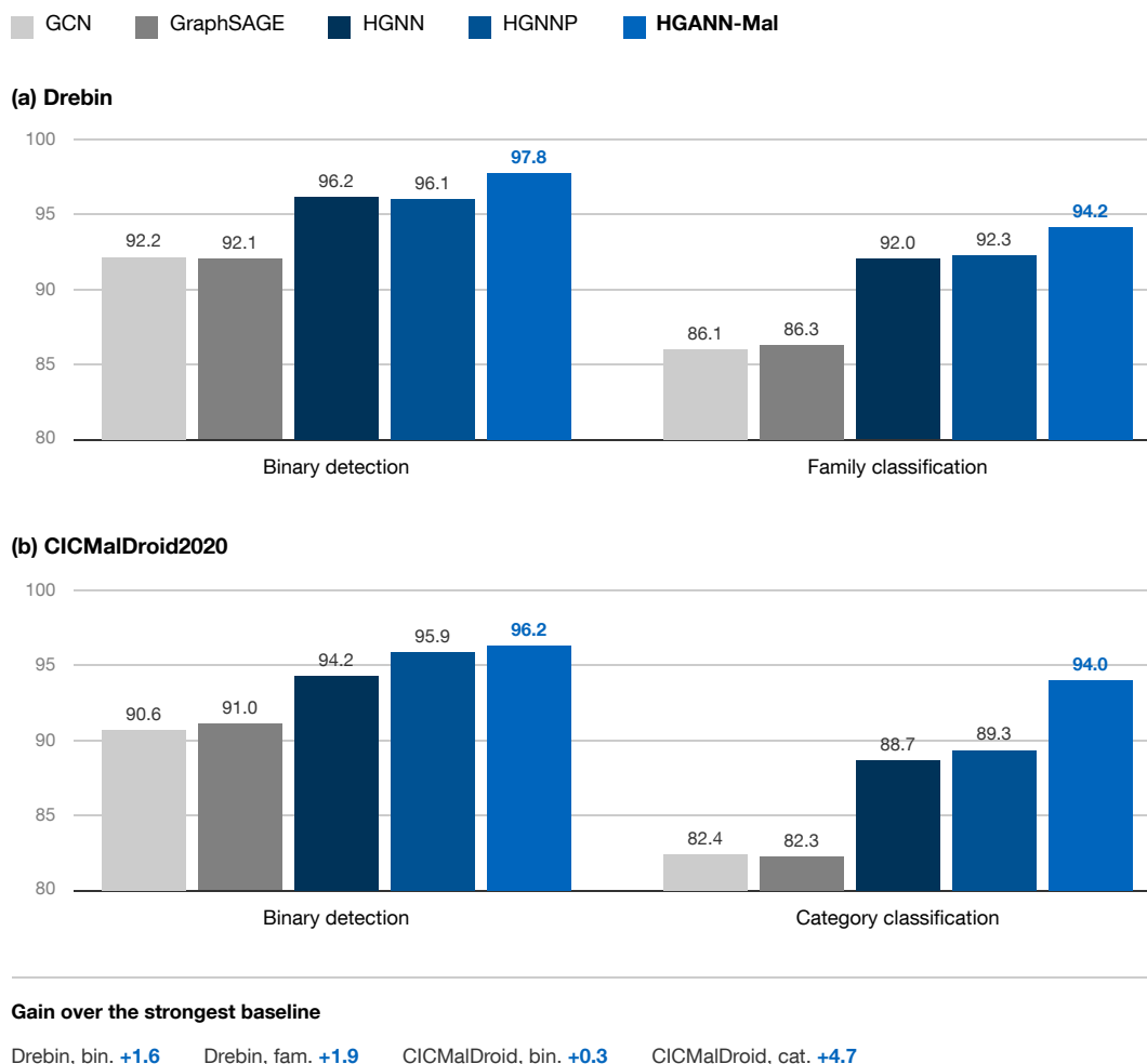
Figure 5.4. F1 on both corpora and both tasks, as published in Tables 5.2 and 5.3. The plot retains the published values, including the Drebin binary discrepancy described in Section 5.10. The source labels them Macro-F1, although several rows cannot follow one averaging convention (Section 5.14). The vertical axis is truncated at 80 so that differences among the hypergraph methods remain visible. HGNNP is the source publication’s name for HGNN+.
