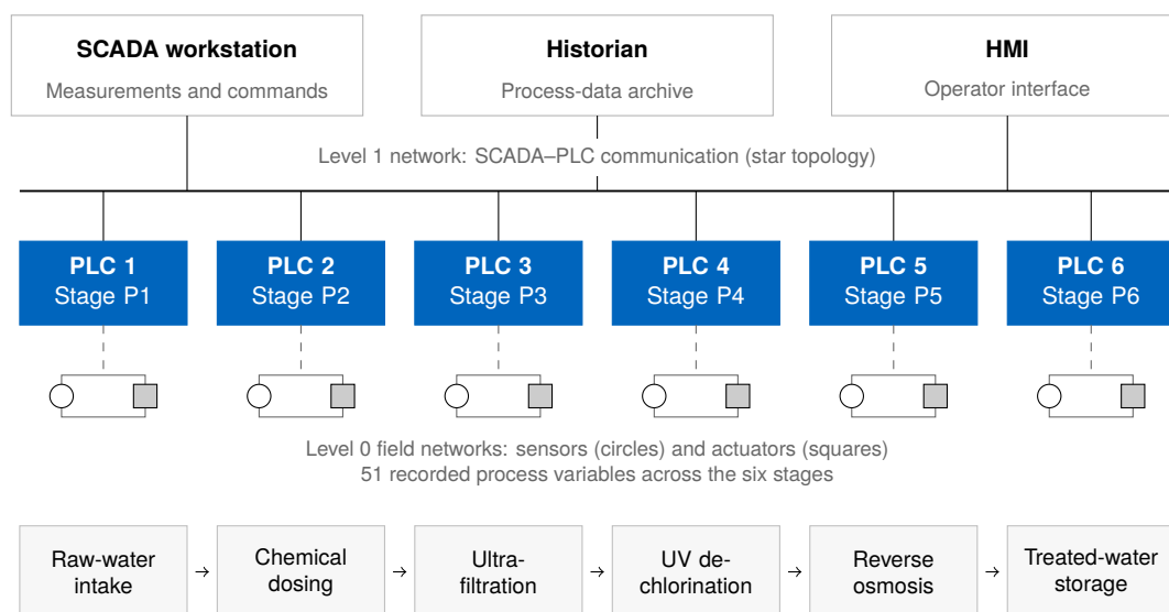
Figure 5.5. SWaT process and control architecture. Network levels follow the SWaT convention. The field-network symbols indicate sensors and actuators within each stage; the detector consumes their recorded values. Adapted from the supplied diagram and the dataset description [34].
