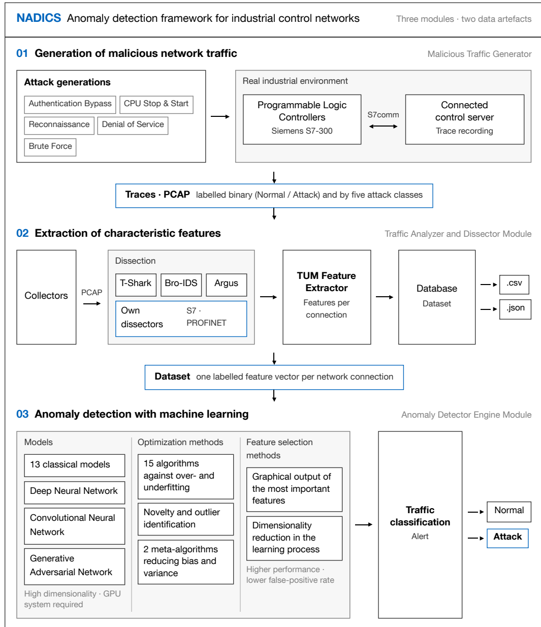
Figure 5.2. Architecture of the NADICS framework. Malicious traffic is generated in a real industrial environment, dissected into protocol-characteristic features, and classified by the anomaly detection engine. The stage structure follows the one reported in the IUNO deliverable [26].
