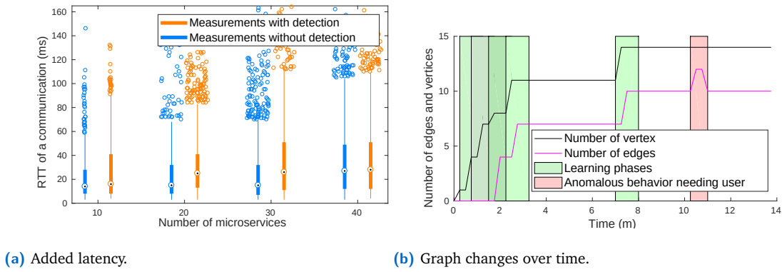
Figure 5.1. The two measurements reported for the service-graph design. Panel (a) gives the inter-service round-trip time with and without detection for ten to forty services. Panel (b) gives the vertex and edge counts of one node's graph over a single run, with the learning phases and the interval of anomalous behaviour shaded. Reproduced from [7], to whose measurement design the candidate contributed.
