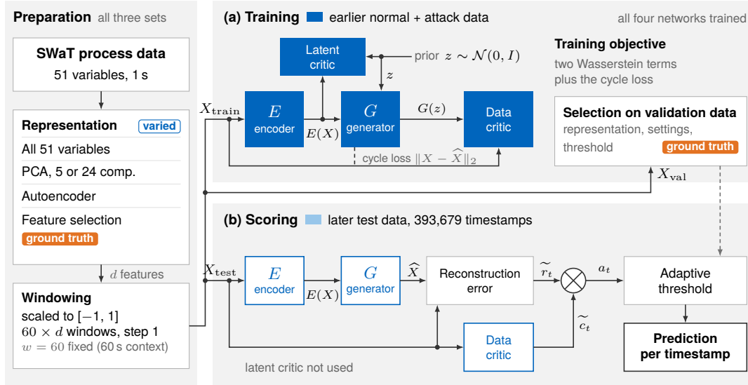
Figure 5.8. Multivariate GAN detection pipeline. (a) The four networks are trained together on earlier windows containing normal and attack observations; validation data select the representation, the settings and the threshold. (b) The later 393,679 test timestamps are scored with the trained networks; the latent critic has no part in the score a_t of Equation 5.1. The blue tag marks the input representation, the only factor varied between runs, and orange tags mark the steps that used attack ground truth. The window length is fixed at 60 samples. The scaler and PCA are fitted on training data and reused for validation and testing. The candidate implemented every processing step shown.
