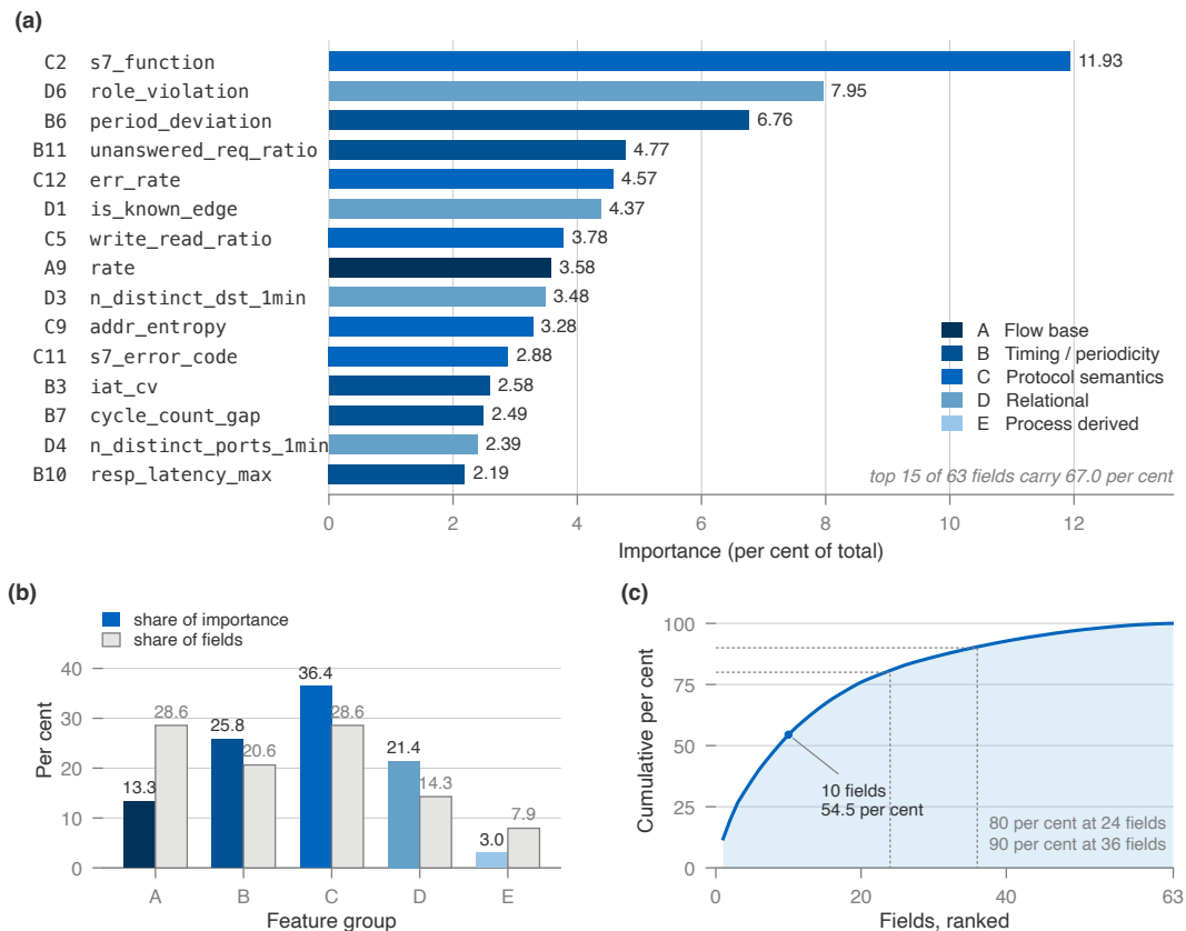
Figure 5.4. Random-forest importance of the 63 extraction fields. (a) The fifteen most important fields, coloured by group. (b) Each group's share of the total importance against its share of the field count. (c) Cumulative share over the ranked fields.
